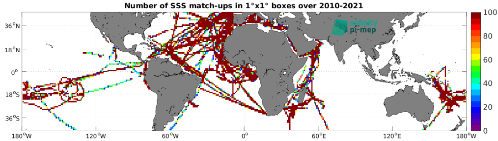
Figure 5: Number of SSS match-ups between TSG (GOSUD-Research-vessel) SSS and the CCI SSS L4 Merged-OI v4.41 - 7-day running (ESA) SSS product for the Mid-Low Latitudes 45N-45S Pi-MEP region over 1^\circ \times 1^\circ boxes and for the full satellite product period.
