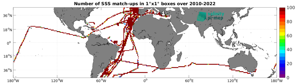
Figure 5: Number of SSS match-ups between TSG (CSIC-UTM) SSS and the CCI SSS L4 Merged-OI v4.41 - 7-day running (ESA) SSS product for the Mid-Low Latitudes 45N-45S Pi-MEP region over 1^\circ \times 1^\circ boxes and for the full satellite product period.
