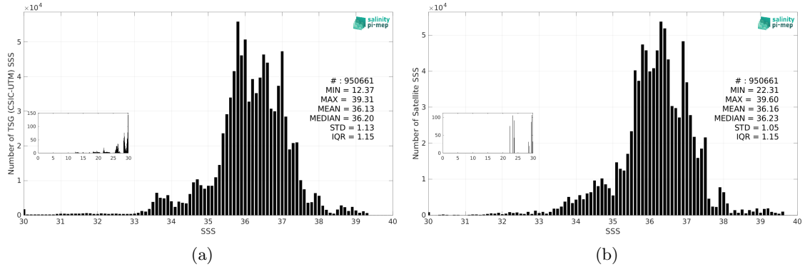
Figure 3: Histograms of SSS from TSG (CSIC-UTM) (a) and CCI SSS L4 Merged-OI v4.41 - 7-day running (ESA) (b) considering all match-up pairs per bins of 0.1 over the Mid-Low Latitudes 45N-45S Pi-MEP region and for the full satellite product period.
