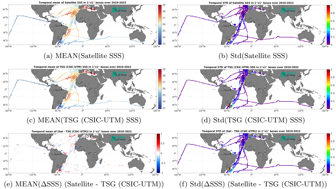
Figure 7: Temporal mean (left) and Std (right) of SSS from CCI SSS L4 Merged-OI v4.41 - 7-day running (ESA) (top), TSG (CSIC-UTM) (middle), and of \Delta SSS (Satellite - TSG (CSIC-UTM)). Only match-up pairs are used to generate these maps.
