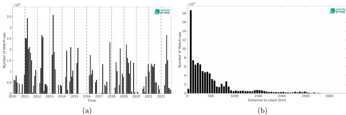
Figure 2: Number of match-ups between TSG (CSIC-UTM) and CCI SSS L4 Merged-OI v4.41 - 7-day running (ESA) SSS as a function of time (a) and as function of the distance to coast (b) over the Mid-Low Latitudes 45N-45S Pi-MEP region and for the full satellite product period.
