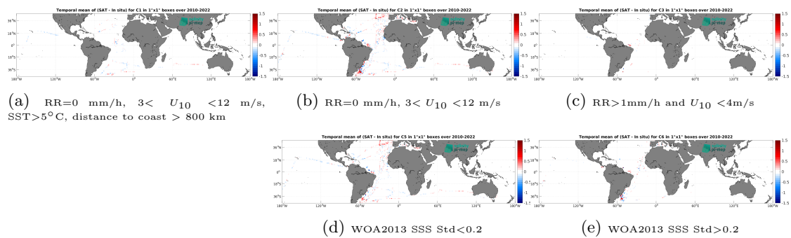
Figure 14: Temporal mean gridded over spatial boxes of size 1^\circ \times 1^\circ of \Delta SSS (CCI SSS L4 Merged-OI v4.41 - 7-day running (ESA) - TSG (CSIC-UTM)) for 5 different subdatasets corresponding to:RR=0 mm/h, 3 < U_{10} < 12 m/s, SST > 5^\circ\text{C} , distance to coast > 800 km (a), RR=0 mm/h, 3 < U_{10} < 12 m/s (b), RR > 1 mm/h and U_{10} < 4 m/s (c), WOA2013 SSS Std < 0.2 (d), WOA2013 SSS Std > 0.2 (e).
