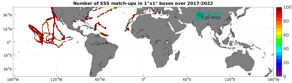
Figure 5: Number of SSS match-ups between Saildrone SSS and the CCI SSS L4 Merged-OI v4.41 - 7-day running (ESA) SSS product for the Mid-Low Latitudes 45N-45S Pi-MEP region over 1^\circ \times 1^\circ boxes and for the full satellite product period.
