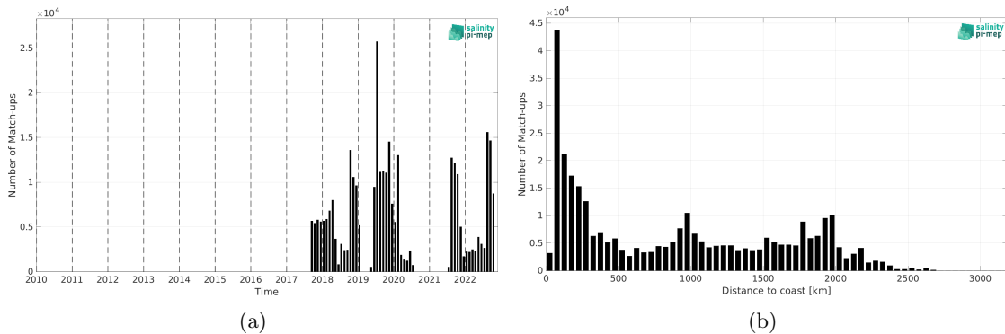
Figure 2: Number of match-ups between Saildrone and CCI SSS L4 Merged-OI v4.41 - 7-day running (ESA) SSS as a function of time (a) and as function of the distance to coast (b) over the Mid-Low Latitudes 45N-45S Pi-MEP region and for the full satellite product period.
