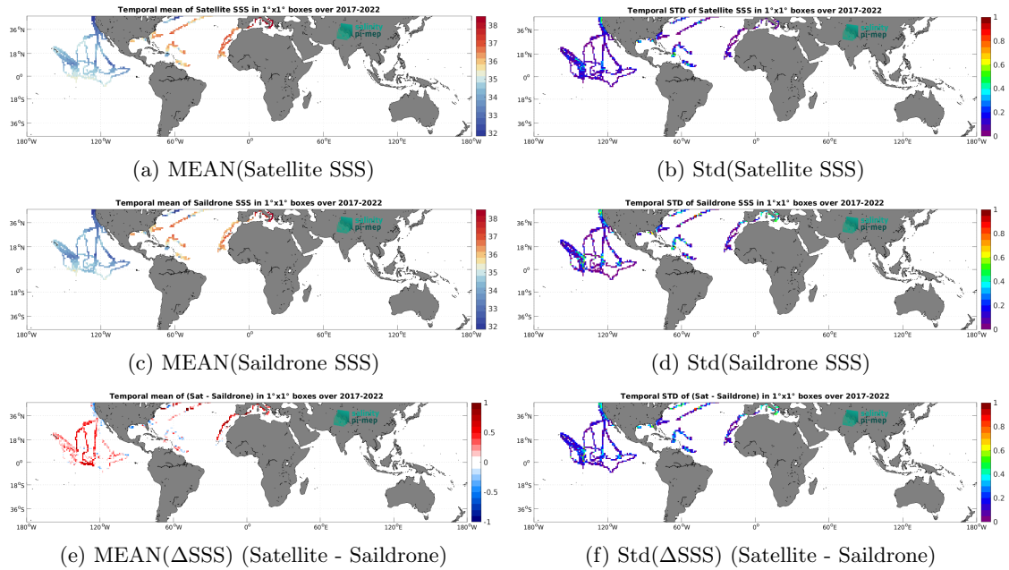
Figure 7: Temporal mean (left) and Std (right) of SSS from CCI SSS L4 Merged-OI v4.41 - 7-day running (ESA) (top), Saildrone (middle), and of \Delta SSS (Satellite - Saildrone). Only match-up pairs are used to generate these maps.
