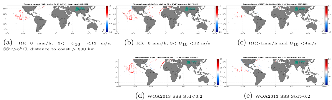
Figure 14: Temporal mean gridded over spatial boxes of size 1^\circ \times 1^\circ of \Delta\text{SSS} (CCI SSS L4 Merged-OI v4.41 - 7-day running (ESA) - Saildrone) for 5 different subdatasets corresponding to: RR=0 mm/h, 3 < U_{10} < 12 m/s, SST > 5°C, distance to coast > 800 km (a), RR=0 mm/h, 3 < U_{10} < 12 m/s (b), RR > 1mm/h and U_{10} < 4 m/s (c), WOA2013 SSS Std < 0.2 (d), WOA2013 SSS Std > 0.2 (e).
