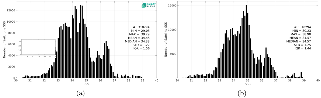
Figure 3: Histograms of SSS from Saildrone (a) and CCI SSS L4 Merged-OI v4.41 - 7-day running (ESA) (b) considering all match-up pairs per bins of 0.1 over the Mid-Low Latitudes 45N-45S Pi-MEP region and for the full satellite product period.
