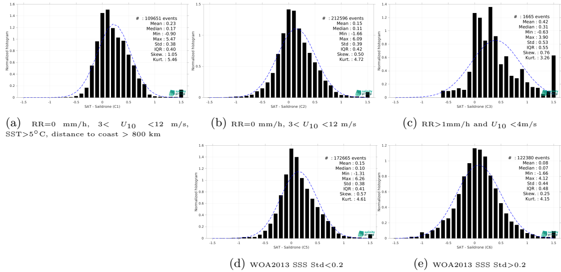
Figure 15: Normalized histogram of \Delta SSS (CCI SSS L4 Merged-OI v4.41 - 7-day running (ESA) - Saildrone) for 5 different subdatasets corresponding to: RR=0 mm/h, 3 < U_{10} < 12 m/s, SST >5^{\circ} C, distance to coast > 800 km (a), RR=0 mm/h, 3 < U_{10} < 12 m/s (b), RR >1 mm/h and U_{10} < 4 m/s (c), WOA2013 SSS Std <0.2 (d), WOA2013 SSS Std >0.2 (e).
