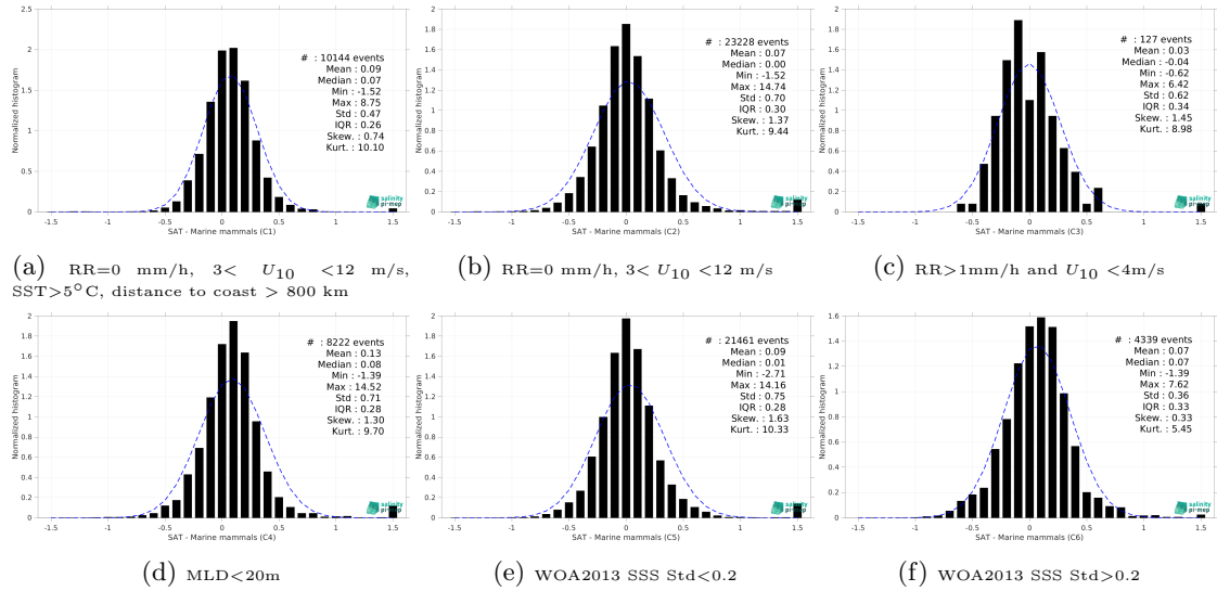
Figure 15: Normalized histogram of \Delta SSS (CCI SSS L4 Merged-OI v4.41 - 7-day running (ESA) - Marine mammals) for 6 different subdatasets corresponding to: RR=0 mm/h, 3 < U_{10} < 12 m/s, SST > 5°C, distance to coast > 800 km (a), RR=0 mm/h, 3 < U_{10} < 12 m/s (b), RR > 1mm/h and U_{10} < 4 m/s (c), MLD < 20m (d), WOA2013 SSS Std < 0.2 (e), WOA2013 SSS Std > 0.2 (f).
