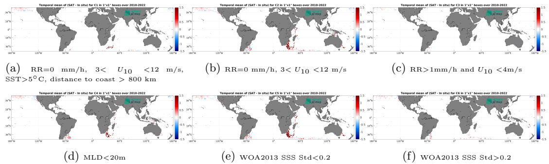
Figure 14: Temporal mean gridded over spatial boxes of size 1^\circ \times 1^\circ of \Delta SSS (CCI SSS L4 Merged-OI v4.41 - 7-day running (ESA) - Marine mammals) for 6 different subdatasets corresponding to:RR=0 mm/h, 3 < U_{10} < 12 m/s, SST > 5°C, distance to coast > 800 km (a), RR=0 mm/h, 3 < U_{10} < 12 m/s (b), RR > 1mm/h and U_{10} < 4 m/s (c),MLD < 20m (d),WOA2013 SSS Std < 0.2 (e),WOA2013 SSS Std > 0.2 (f).
