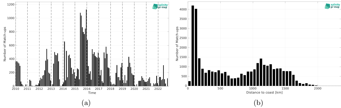
Figure 2: Number of match-ups between Marine mammals and CCI SSS L4 Merged-OI v4.41 - 7-day running (ESA) SSS as a function of time (a) and as function of the distance to coast (b) over the Mid-Low Latitudes 45N-45S Pi-MEP region and for the full satellite product period.
