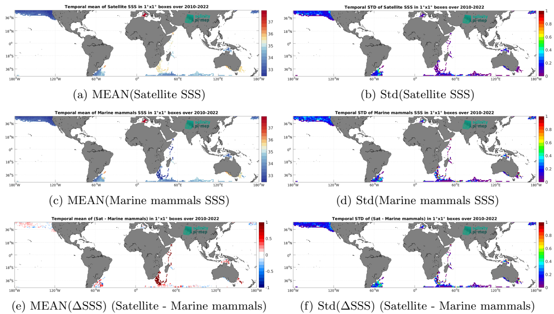
Figure 7: Temporal mean (left) and Std (right) of SSS from CCI SSS L4 Merged-OI v4.41 - 7-day running (ESA) (top), Marine mammals (middle), and of \Delta SSS (Satellite - Marine mammals). Only match-up pairs are used to generate these maps.
