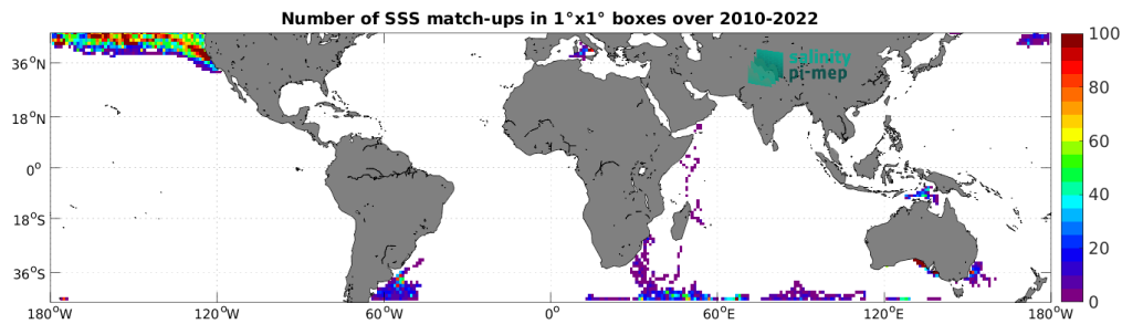
Figure 5: Number of SSS match-ups between Marine mammals SSS and the CCI SSS L4 Merged-OI v4.41 - 7-day running (ESA) SSS product for the Mid-Low Latitudes 45N-45S Pi-MEP region over 1^\circ \times 1^\circ boxes and for the full satellite product period.
