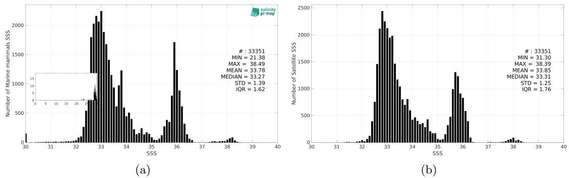
Figure 3: Histograms of SSS from Marine mammals (a) and CCI SSS L4 Merged-OI v4.41 - 7-day running (ESA) (b) considering all match-up pairs per bins of 0.1 over the Mid-Low Latitudes 45N-45S Pi-MEP region and for the full satellite product period.
