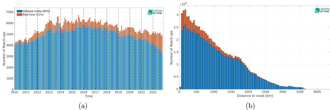
Figure 2: Number of match-ups between Argo and CCI SSS L4 Merged-OI v4.41 - 7-day running (ESA) SSS as a function of time (a) and as function of the distance to coast (b) over the Mid-Low Latitudes 45N-45S Pi-MEP region and for the full satellite product period.
