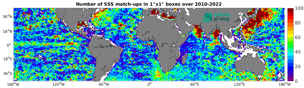
Figure 5: Number of SSS match-ups between Argo SSS and the CCI SSS L4 Merged-OI v4.41 - 7-day running (ESA) SSS product for the Mid-Low Latitudes 45N-45S Pi-MEP region over 1^\circ \times 1^\circ boxes and for the full satellite product period.
