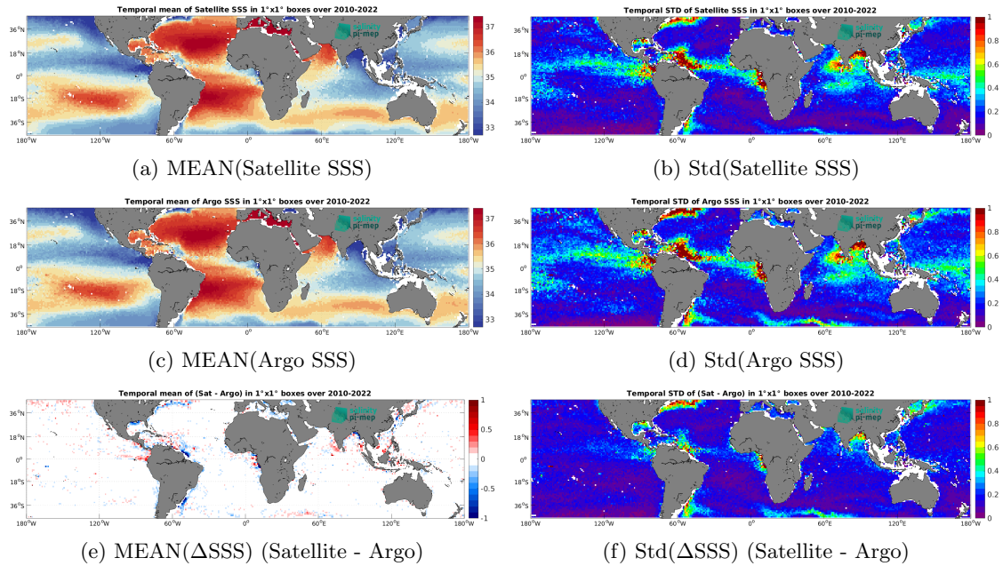
Figure 7: Temporal mean (left) and Std (right) of SSS from CCI SSS L4 Merged-OI v4.41 - 7-day running (ESA) (top), Argo (middle), and of \Delta SSS (Satellite - Argo). Only match-up pairs are used to generate these maps.
