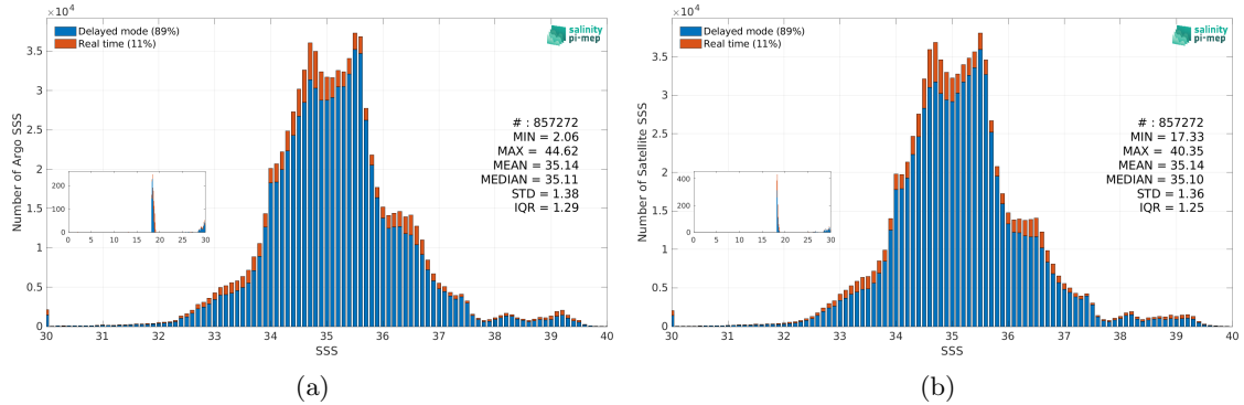
Figure 3: Histograms of SSS from Argo (a) and CCI SSS L4 Merged-OI v4.41 - 7-day running (ESA) (b) considering all match-up pairs per bins of 0.1 over the Mid-Low Latitudes 45N-45S Pi-MEP region and for the full satellite product period.
