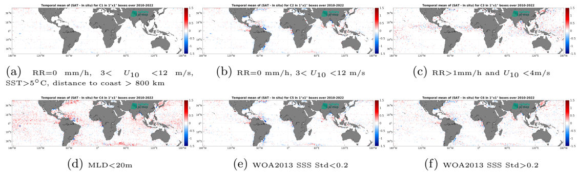
Figure 14: Temporal mean gridded over spatial boxes of size 1^\circ \times 1^\circ of \Delta SSS (CCI SSS L4 Merged-OI v4.41 - 7-day running (ESA) - Argo) for 6 different subdatasets corresponding to:RR=0 mm/h, 3 < U_{10} < 12 m/s, SST >5^\circ C, distance to coast > 800 km (a), RR=0 mm/h, 3 < U_{10} < 12 m/s (b), RR >1 mm/h and U_{10} < 4 m/s (c),MLD <20 m (d),WOA2013 SSS Std <0.2 (e),WOA2013 SSS Std >0.2 (f).
