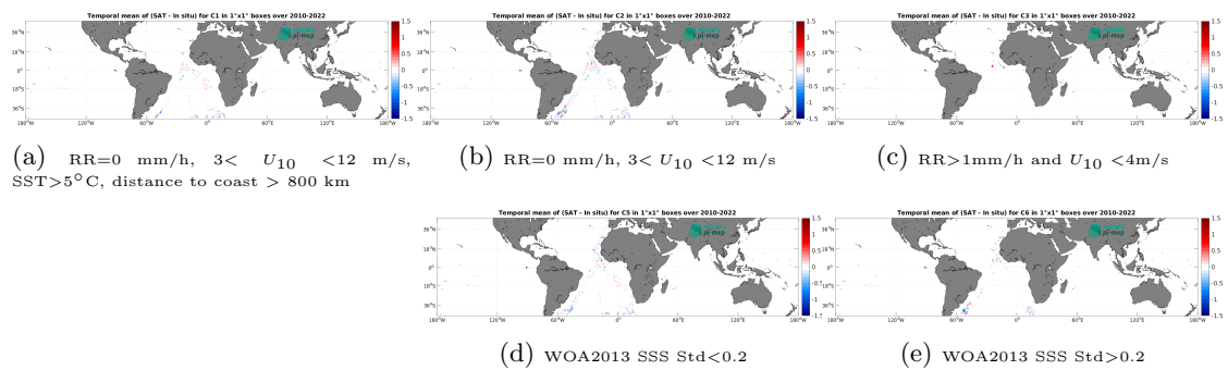
Figure 14: Temporal mean gridded over spatial boxes of size 1^\circ \times 1^\circ of \Delta SSS (CCI SSS L4 Merged-OI v4.41 - 30-day running (ESA) - TSG (Polarstern)) for 5 different subdatasets corresponding to:RR=0 mm/h, 3 < U_{10} < 12 m/s, SST >5^\circ C, distance to coast > 800 km (a), RR=0 mm/h, 3 < U_{10} < 12 m/s (b), RR >1 mm/h and U_{10} < 4 m/s (c), WOA2013 SSS Std <0.2 (d), WOA2013 SSS Std >0.2 (e).
