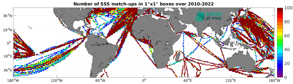
Figure 5: Number of SSS match-ups between TSG (LEGOS-DM) SSS and the CCI SSS L4 Merged-OI v4.41 - 30-day running (ESA) SSS product for the Mid-Low Latitudes 45N-45S Pi-MEP region over 1^\circ \times 1^\circ boxes and for the full satellite product period.
