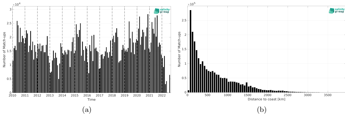
Figure 2: Number of match-ups between TSG (LEGOS-DM) and CCI SSS L4 Merged-OI v4.41 - 30-day running (ESA) SSS as a function of time (a) and as function of the distance to coast (b) over the Mid-Low Latitudes 45N-45S Pi-MEP region and for the full satellite product period.
