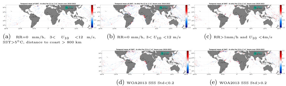
Figure 14: Temporal mean gridded over spatial boxes of size 1^\circ \times 1^\circ of \Delta\text{SSS} (CCI SSS L4 Merged-OI v4.41 - 30-day running (ESA) - TSG (LEGOS-DM)) for 5 different subdatasets corresponding to:RR=0 mm/h, 3 < U_{10} < 12 m/s, SST >5^\circ\text{C} , distance to coast > 800 km (a), RR=0 mm/h, 3 < U_{10} < 12 m/s (b), RR >1 mm/h and U_{10} < 4 m/s (c), WOA2013 SSS Std <0.2 (d), WOA2013 SSS Std >0.2 (e).
