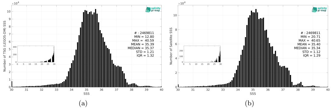
Figure 3: Histograms of SSS from TSG (LEGOS-DM) (a) and CCI SSS L4 Merged-OI v4.41 - 30-day running (ESA) (b) considering all match-up pairs per bins of 0.1 over the Mid-Low Latitudes 45N-45S Pi-MEP region and for the full satellite product period.
