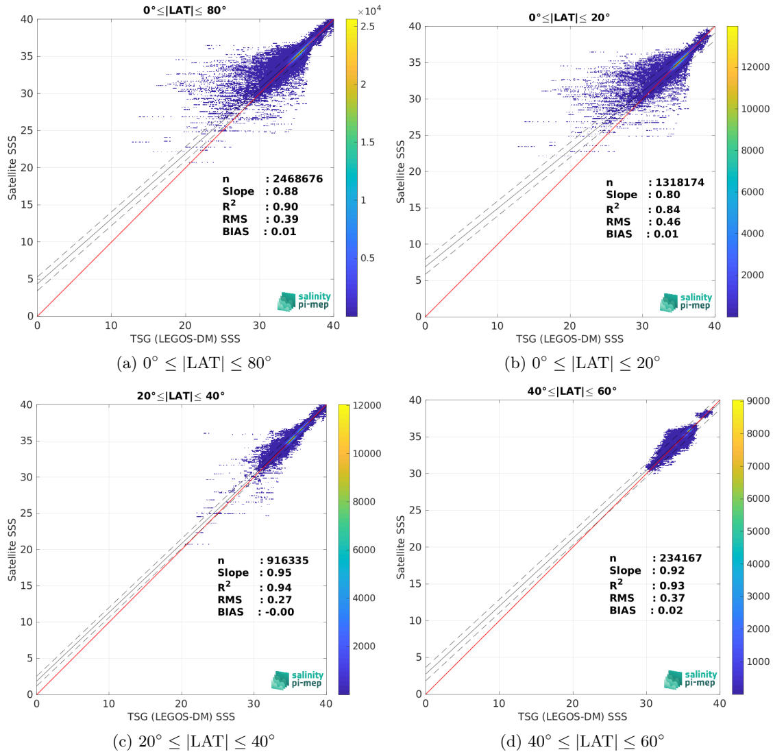
Figure 10: Contour maps of the concentration of CCI SSS L4 Merged-OI v4.41 - 30-day running (ESA) SSS (y-axis) versus TSG (LEGOS-DM) SSS (x-axis) at match-up pairs for different latitude bands. For each plot, the red line shows x=y . The black thin and dashed lines indicate a linear fit through the data cloud and the \pm 95\% confidence levels, respectively. The number match-up pairs n , the slope and R^2 coefficient of the linear fit, the root mean square (RMS) and the mean bias between satellite and in situ data are indicated for each latitude band in each plots.
