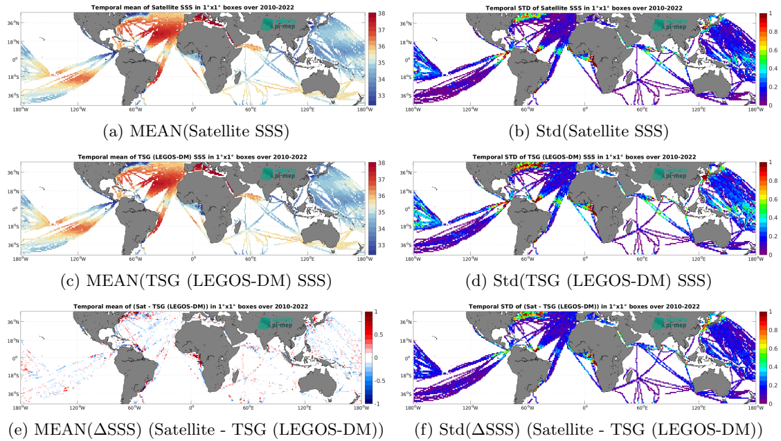
Figure 7: Temporal mean (left) and Std (right) of SSS from CCI SSS L4 Merged-OI v4.41 - 30-day running (ESA) (top), TSG (LEGOS-DM) (middle), and of \Delta SSS (Satellite - TSG (LEGOS-DM)). Only match-up pairs are used to generate these maps.
