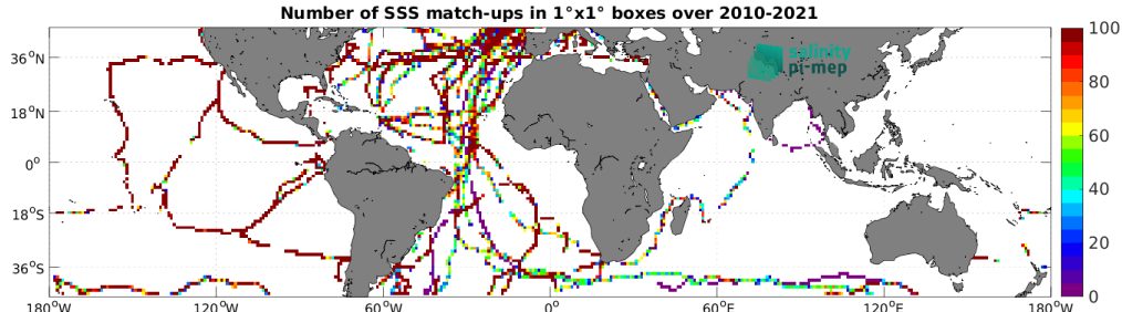
Figure 5: Number of SSS match-ups between TSG (GOSUD-Sailing-ship) SSS and the CCI SSS L4 Merged-OI v4.41 - 30-day running (ESA) SSS product for the Mid-Low Latitudes 45N-45S Pi-MEP region over 1^\circ \times 1^\circ boxes and for the full satellite product period.
