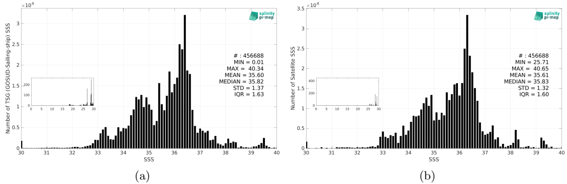
Figure 3: Histograms of SSS from TSG (GOSUD-Sailing-ship) (a) and CCI SSS L4 Merged-OI v4.41 - 30-day running (ESA) (b) considering all match-up pairs per bins of 0.1 over the Mid-Low Latitudes 45N-45S Pi-MEP region and for the full satellite product period.
