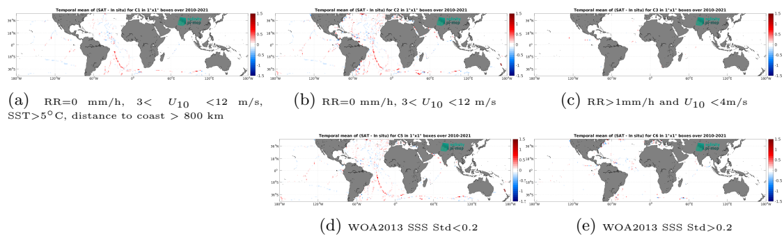
Figure 14: Temporal mean gridded over spatial boxes of size 1^\circ \times 1^\circ of \Delta SSS (CCI SSS L4 Merged-OI v4.41 - 30-day running (ESA) - TSG (GOSUD-Sailing-ship)) for 5 different subdatasets corresponding to: RR=0 mm/h, 3 < U_{10} < 12 m/s, SST > 5^\circ\text{C} , distance to coast > 800 km (a), RR=0 mm/h, 3 < U_{10} < 12 m/s (b), RR > 1 mm/h and U_{10} < 4 m/s (c), WOA2013 SSS Std < 0.2 (d), WOA2013 SSS Std > 0.2 (e).
