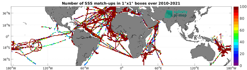
Figure 5: Number of SSS match-ups between TSG (GOSUD-Research-vessel) SSS and the CCI SSS L4 Merged-OI v4.41 - 30-day running (ESA) SSS product for the Mid-Low Latitudes 45N-45S Pi-MEP region over 1^{\circ} \times 1^{\circ} boxes and for the full satellite product period.
