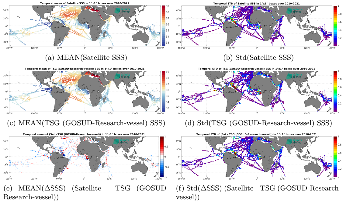
Figure 7: Temporal mean (left) and Std (right) of SSS from CCI SSS L4 Merged-OI v4.41 - 30-day running (ESA) (top), TSG (GOSUD-Research-vessel) (middle), and of \Delta SSS (Satellite - TSG (GOSUD-Research-vessel)). Only match-up pairs are used to generate these maps.
