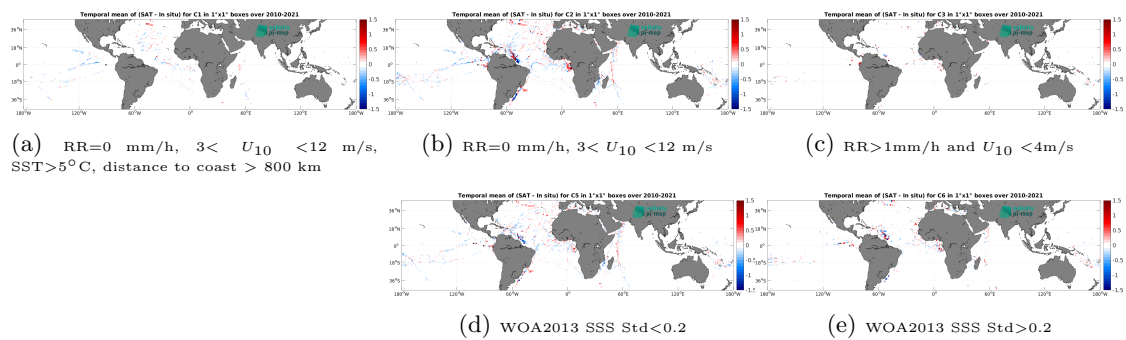
Figure 14: Temporal mean gridded over spatial boxes of size 1^\circ \times 1^\circ of \Delta SSS (CCI SSS L4 Merged-OI v4.41 - 30-day running (ESA) - TSG (GOSUD-Research-vessel)) for 5 different subdatasets corresponding to: RR=0 mm/h, 3 < U_{10} < 12 m/s, SST > 5^\circ\text{C} , distance to coast > 800 km (a), RR=0 mm/h, 3 < U_{10} < 12 m/s (b), RR > 1 mm/h and U_{10} < 4 m/s (c), WOA2013 SSS Std < 0.2 (d), WOA2013 SSS Std > 0.2 (e).
