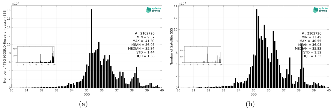
Figure 3: Histograms of SSS from TSG (GOSUD-Research-vessel) (a) and CCI SSS L4 Merged-OI v4.41 - 30-day running (ESA) (b) considering all match-up pairs per bins of 0.1 over the Mid-Low Latitudes 45N-45S Pi-MEP region and for the full satellite product period.
