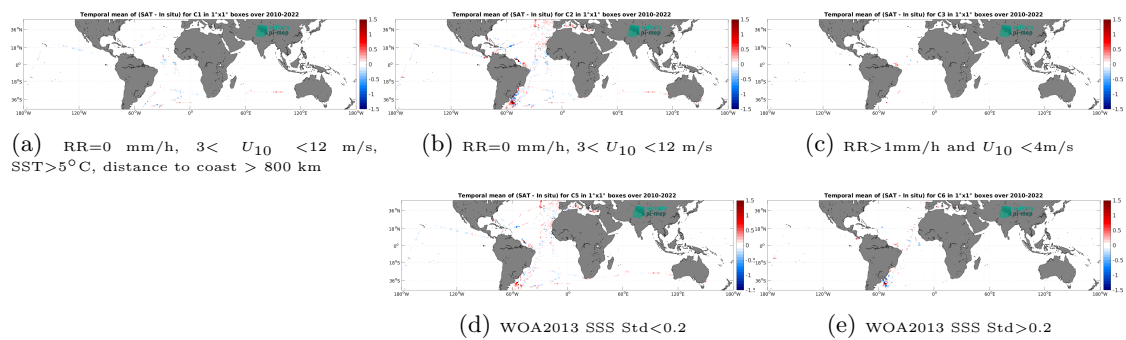
Figure 14: Temporal mean gridded over spatial boxes of size 1^\circ \times 1^\circ of \Delta\text{SSS} (CCI SSS L4 Merged-OI v4.41 - 30-day running (ESA) - TSG (CSIC-UTM)) for 5 different subdatasets corresponding to:RR=0 mm/h, 3 < U_{10} < 12 m/s, SST > 5°C, distance to coast > 800 km (a), RR=0 mm/h, 3 < U_{10} < 12 m/s (b), RR > 1mm/h and U_{10} < 4 m/s (c), WOA2013 SSS Std < 0.2 (d), WOA2013 SSS Std > 0.2 (e).
