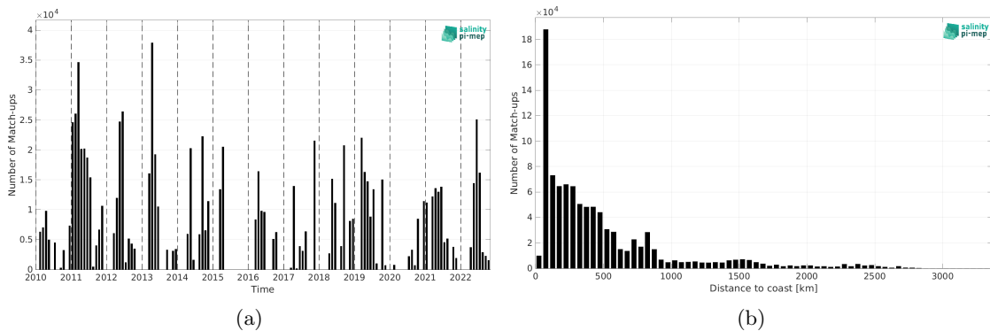
Figure 2: Number of match-ups between TSG (CSIC-UTM) and CCI SSS L4 Merged-OI v4.41 - 30-day running (ESA) SSS as a function of time (a) and as function of the distance to coast (b) over the Mid-Low Latitudes 45N-45S Pi-MEP region and for the full satellite product period.
