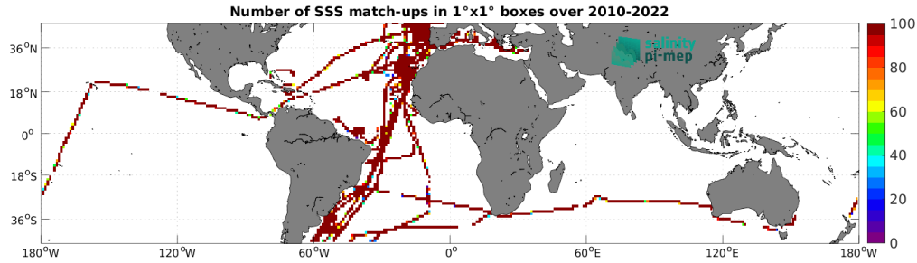
Figure 5: Number of SSS match-ups between TSG (CSIC-UTM) SSS and the CCI SSS L4 Merged-OI v4.41 - 30-day running (ESA) SSS product for the Mid-Low Latitudes 45N-45S Pi-MEP region over 1^\circ \times 1^\circ boxes and for the full satellite product period.
