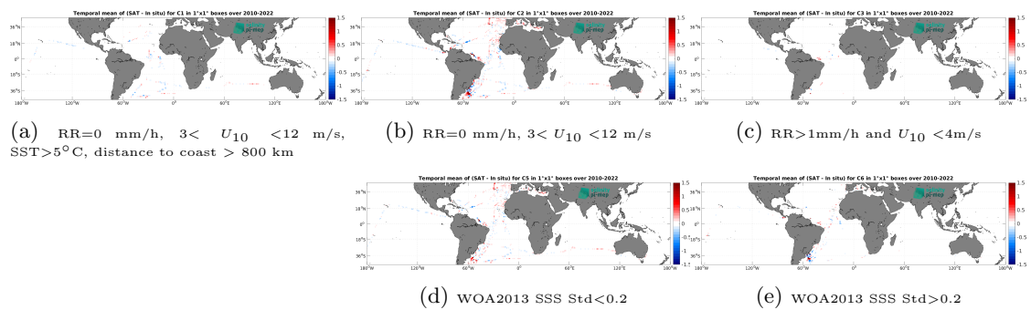
Figure 14: Temporal mean gridded over spatial boxes of size 1^\circ \times 1^\circ of \Delta SSS (CCI SSS L4 Merged-OI v4.41 - 30-day running (ESA) - TSG (CSIC-UTM)) for 5 different subdatasets corresponding to:RR=0 mm/h, 3 < U_{10} < 12 m/s, SST >5^\circ\text{C} , distance to coast > 800 km (a), RR=0 mm/h, 3 < U_{10} < 12 m/s (b), RR >1 mm/h and U_{10} < 4 m/s (c), WOA2013 SSS Std <0.2 (d), WOA2013 SSS Std >0.2 (e).
