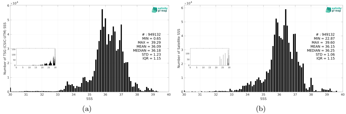
Figure 3: Histograms of SSS from TSG (CSIC-UTM) (a) and CCI SSS L4 Merged-OI v4.41 - 30-day running (ESA) (b) considering all match-up pairs per bins of 0.1 over the Mid-Low Latitudes 45N-45S Pi-MEP region and for the full satellite product period.
