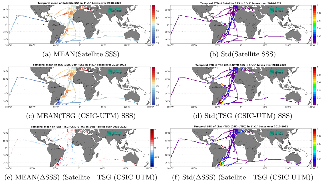
Figure 7: Temporal mean (left) and Std (right) of SSS from CCI SSS L4 Merged-OI v4.41 - 30-day running (ESA) (top), TSG (CSIC-UTM) (middle), and of \Delta SSS (Satellite - TSG (CSIC-UTM)). Only match-up pairs are used to generate these maps.
