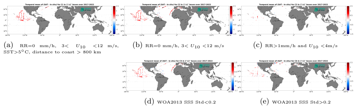
Figure 14: Temporal mean gridded over spatial boxes of size 1^\circ \times 1^\circ of \Delta\text{SSS} (CCI SSS L4 Merged-OI v4.41 - 30-day running (ESA) - Saildrone) for 5 different subdatasets corresponding to:RR=0 mm/h, 3 < U_{10} < 12 m/s, SST>5°C, distance to coast > 800 km (a), RR=0 mm/h, 3 < U_{10} < 12 m/s (b), RR>1mm/h and U_{10} < 4 m/s (c), WOA2013 SSS Std<0.2 (d), WOA2013 SSS Std>0.2 (e).
