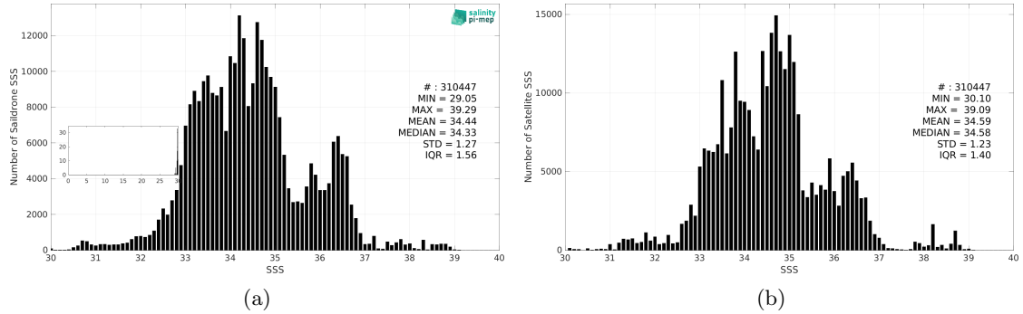
Figure 3: Histograms of SSS from Saildrone (a) and CCI SSS L4 Merged-OI v4.41 - 30-day running (ESA) (b) considering all match-up pairs per bins of 0.1 over the Mid-Low Latitudes 45N-45S Pi-MEP region and for the full satellite product period.
