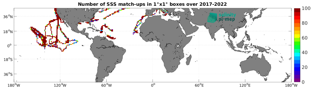
Figure 5: Number of SSS match-ups between Saildrone SSS and the CCI SSS L4 Merged-OI v4.41 - 30-day running (ESA) SSS product for the Mid-Low Latitudes 45N-45S Pi-MEP region over 1^\circ \times 1^\circ boxes and for the full satellite product period.
