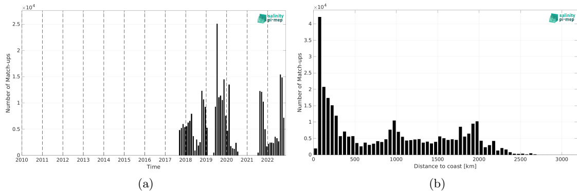
Figure 2: Number of match-ups between Saildrone and CCI SSS L4 Merged-OI v4.41 - 30-day running (ESA) SSS as a function of time (a) and as function of the distance to coast (b) over the Mid-Low Latitudes 45N-45S Pi-MEP region and for the full satellite product period.
