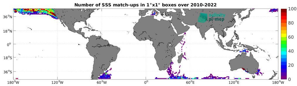
Figure 5: Number of SSS match-ups between Marine mammals SSS and the CCI SSS L4 Merged-OI v4.41 - 30-day running (ESA) SSS product for the Mid-Low Latitudes 45N-45S Pi-MEP region over 1°x1° boxes and for the full satellite product period.
