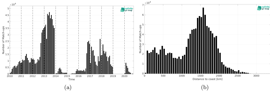
Figure 2: Number of match-ups between Surface drifters and CCI SSS L4 Merged-OI v4.41 - 30-day running (ESA) SSS as a function of time (a) and as function of the distance to coast (b) over the Mid-Low Latitudes 45N-45S Pi-MEP region and for the full satellite product period.
