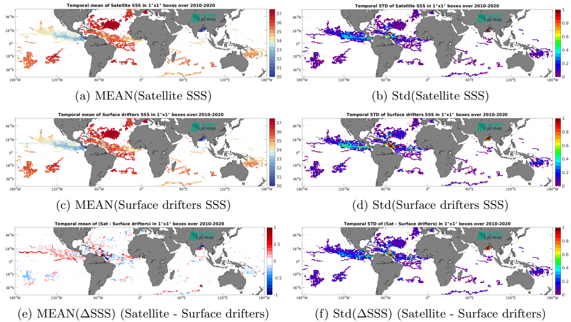
Figure 6: Temporal mean (left) and Std (right) of SSS from CCI SSS L4 Merged-OI v4.41 - 30-day running (ESA) (top), Surface drifters (middle), and of \Delta SSS (Satellite - Surface drifters). Only match-up pairs are used to generate these maps.
