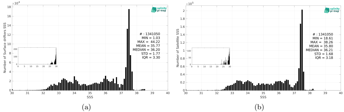
Figure 3: Histograms of SSS from Surface drifters (a) and CCI SSS L4 Merged-OI v4.41 - 30-day running (ESA) (b) considering all match-up pairs per bins of 0.1 over the Mid-Low Latitudes 45N-45S Pi-MEP region and for the full satellite product period.
