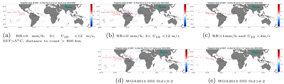
Figure 13: Temporal mean gridded over spatial boxes of size 1^\circ \times 1^\circ of \Delta\text{SSS} (CCI SSS L4 Merged-OI v4.41 - 30-day running (ESA) - Surface drifters) for 5 different subdatasets corresponding to:RR=0 mm/h, 3 < U_{10} < 12 m/s, SST >5^\circ\text{C} , distance to coast > 800 km (a), RR=0 mm/h, 3 < U_{10} < 12 m/s (b), RR >1 mm/h and U_{10} < 4 m/s (c), WOA2013 SSS Std <0.2 (d), WOA2013 SSS Std >0.2 (e).
