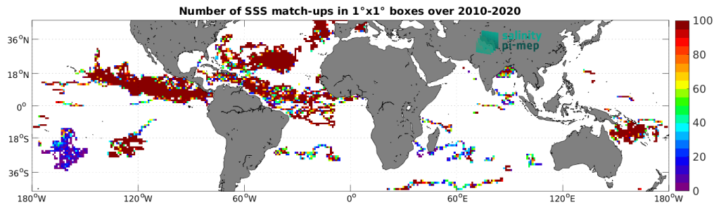
Figure 4: Number of SSS match-ups between Surface drifters SSS and the CCI SSS L4 Merged-OI v4.41 - 30-day running (ESA) SSS product for the Mid-Low Latitudes 45N-45S Pi-MEP region over 1^\circ \times 1^\circ boxes and for the full satellite product period.
