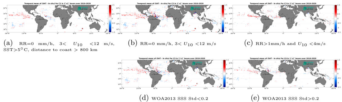
Figure 13: Temporal mean gridded over spatial boxes of size 1^\circ \times 1^\circ of \Delta SSS (CCI SSS L4 Merged-OI v4.41 - 30-day running (ESA) - Surface drifters) for 5 different subdatasets corresponding to:RR=0 mm/h, 3 < U_{10} < 12 m/s, SST >5^\circ C, distance to coast > 800 km (a), RR=0 mm/h, 3 < U_{10} < 12 m/s (b), RR >1 mm/h and U_{10} < 4 m/s (c), WOA2013 SSS Std <0.2 (d), WOA2013 SSS Std >0.2 (e).
