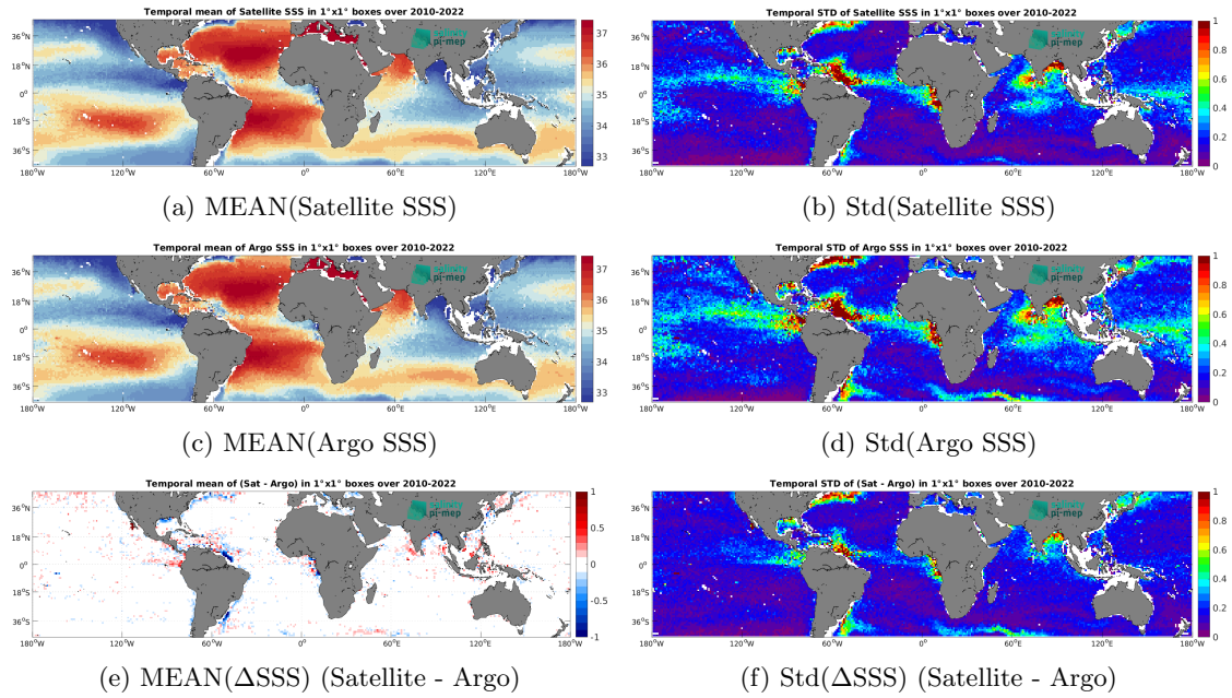
Figure 7: Temporal mean (left) and Std (right) of SSS from CCI SSS L4 Merged-OI v4.41 - 30-day running (ESA) (top), Argo (middle), and of \Delta SSS (Satellite - Argo). Only match-up pairs are used to generate these maps.
