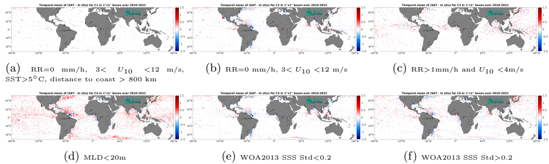
Figure 14: Temporal mean gridded over spatial boxes of size 1^\circ \times 1^\circ of \Delta\text{SSS} (CCI SSS L4 Merged-OI v4.41 - 30-day running (ESA) - Argo) for 6 different subdatasets corresponding to:RR=0 mm/h, 3 < U_{10} < 12 m/s, SST>5°C, distance to coast > 800 km (a), RR=0 mm/h, 3 < U_{10} < 12 m/s (b), RR>1mm/h and U_{10} < 4 m/s (c),MLD<20m (d),WOA2013 SSS Std<0.2 (e),WOA2013 SSS Std>0.2 (f).
