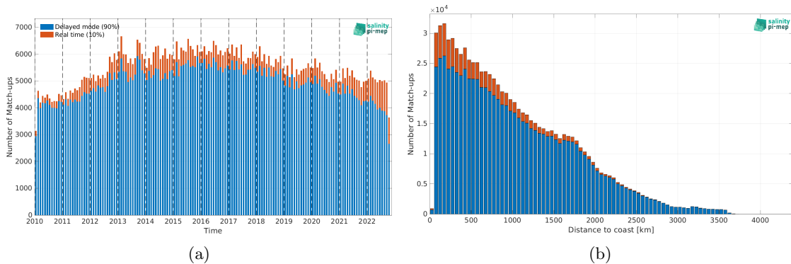
Figure 2: Number of match-ups between Argo and CCI SSS L4 Merged-OI v4.41 - 30-day running (ESA) SSS as a function of time (a) and as function of the distance to coast (b) over the Mid-Low Latitudes 45N-45S Pi-MEP region and for the full satellite product period.
