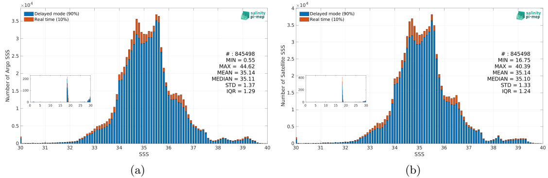
Figure 3: Histograms of SSS from Argo (a) and CCI SSS L4 Merged-OI v4.41 - 30-day running (ESA) (b) considering all match-up pairs per bins of 0.1 over the Mid-Low Latitudes 45N-45S Pi-MEP region and for the full satellite product period.
