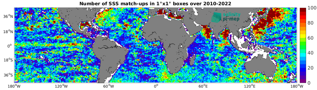
Figure 5: Number of SSS match-ups between Argo SSS and the CCI SSS L4 Merged-OI v4.41 - 30-day running (ESA) SSS product for the Mid-Low Latitudes 45N-45S Pi-MEP region over 1^\circ \times 1^\circ boxes and for the full satellite product period.
