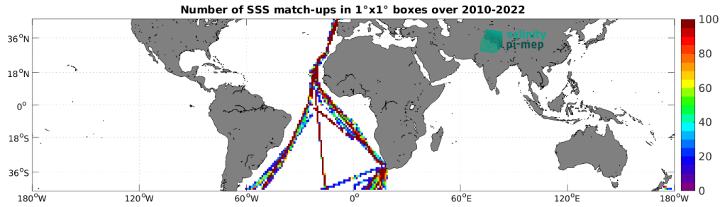
Figure 4: Number of SSS match-ups between TSG (Polarstern) SSS and the CCI SSS L4 Merged-OI v4.4 - 7-day running (ESA) SSS product for the Mid-Low Latitudes 45N-45S Pi-MEP region over 1^\circ \times 1^\circ boxes and for the full satellite product period.
