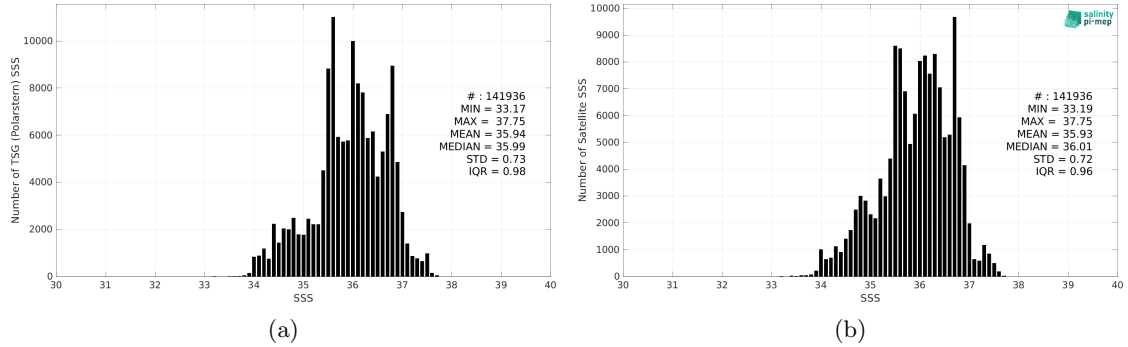
Figure 2: Histograms of SSS from TSG (Polarstern) (a) and CCI SSS L4 Merged-OI v4.4 - 7-day running (ESA) (b) considering all match-up pairs per bins of 0.1 over the Mid-Low Latitudes 45N-45S Pi-MEP region and for the full satellite product period.
