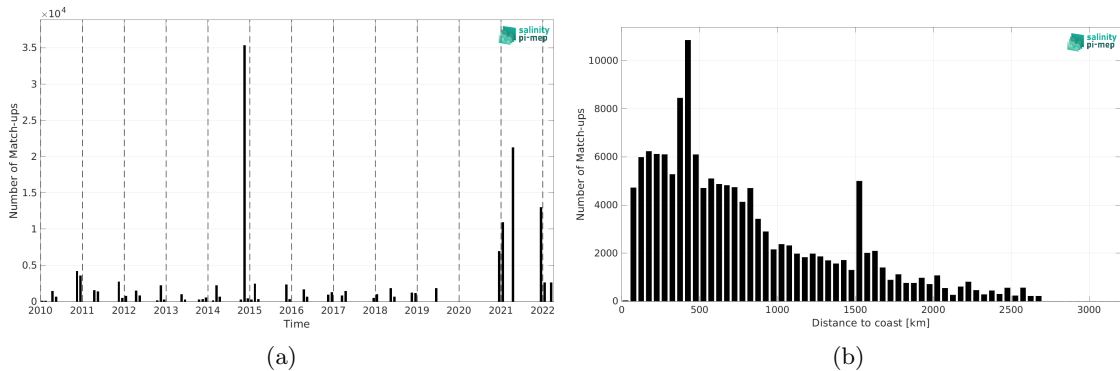
Figure 1: Number of match-ups between TSG (Polarstern) and CCI SSS L4 Merged-OI v4.4 - 7-day running (ESA) SSS as a function of time (a) and as function of the distance to coast (b) over the Mid-Low Latitudes 45N-45S Pi-MEP region and for the full satellite product period.
