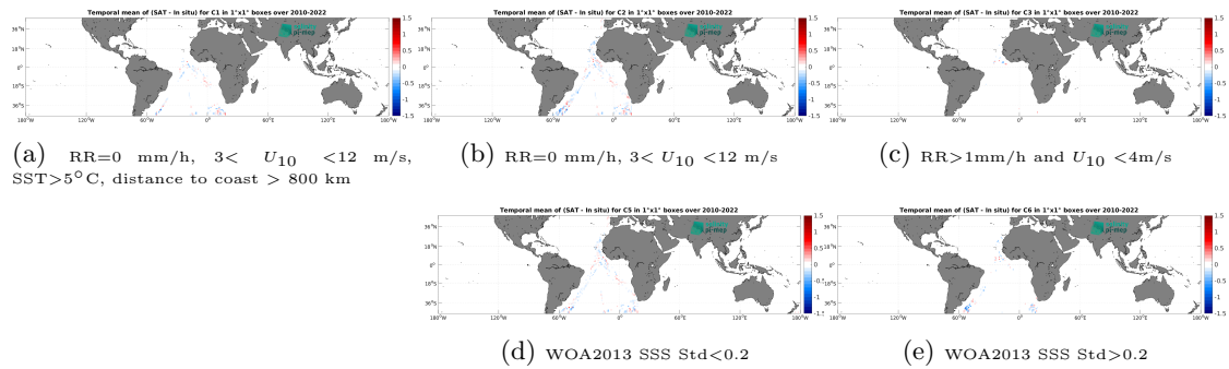
Figure 12: Temporal mean gridded over spatial boxes of size 1^\circ \times 1^\circ of \Delta SSS (CCI SSS L4 Merged-OI v4.4 - 7-day running (ESA) - TSG (Polarstern)) for 5 different subdatasets corresponding to:RR=0 mm/h, 3 < U_{10} < 12 m/s, SST >5^\circ C, distance to coast > 800 km (a), RR=0 mm/h, 3 < U_{10} < 12 m/s (b), RR >1 mm/h and U_{10} < 4 m/s (c), WOA2013 SSS Std <0.2 (d), WOA2013 SSS Std >0.2 (e).
