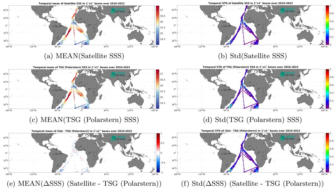
Figure 6: Temporal mean (left) and Std (right) of SSS from CCI SSS L4 Merged-OI v4.4 - 7-day running (ESA) (top), TSG (Polarstern) (middle), and of \Delta SSS (Satellite - TSG (Polarstern)). Only match-up pairs are used to generate these maps.
