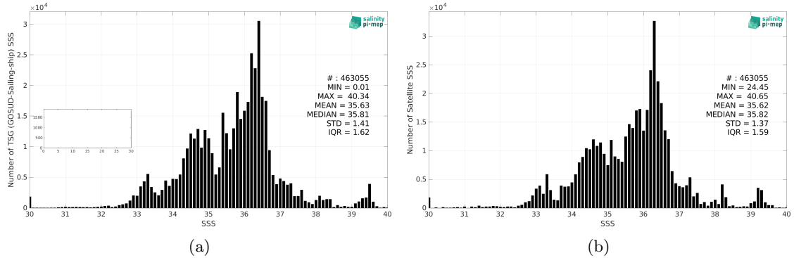
Figure 2: Histograms of SSS from TSG (GOSUD-Sailing-ship) (a) and CCI SSS L4 Merged-OI v4.4 - 7-day running (ESA) (b) considering all match-up pairs per bins of 0.1 over the Mid-Low Latitudes 45N-45S Pi-MEP region and for the full satellite product period.
