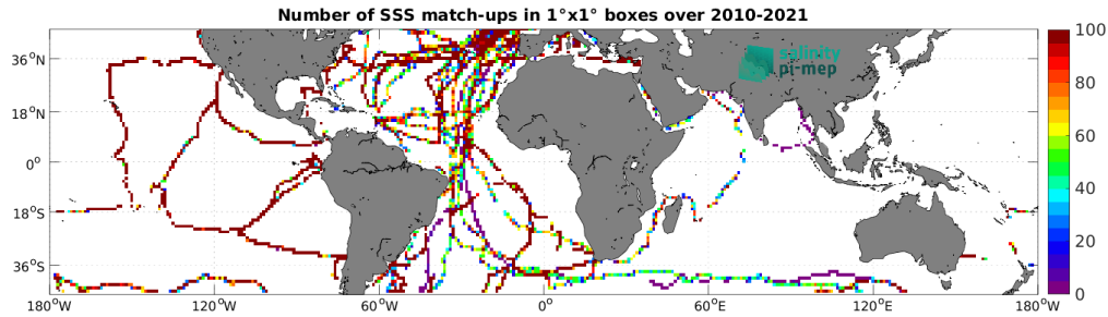
Figure 4: Number of SSS match-ups between TSG (GOSUD-Sailing-ship) SSS and the CCI SSS L4 Merged-OI v4.4 - 7-day running (ESA) SSS product for the Mid-Low Latitudes 45N-45S Pi-MEP region over 1^{\circ} \times 1^{\circ} boxes and for the full satellite product period.
