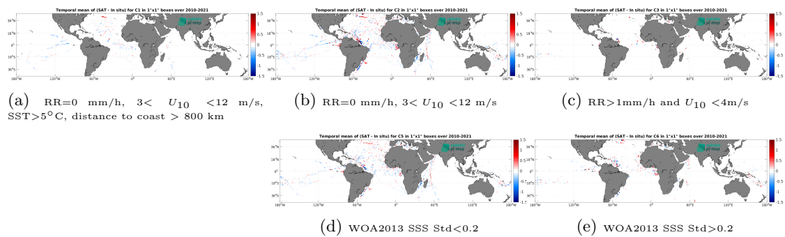
Figure 12: Temporal mean gridded over spatial boxes of size 1^\circ \times 1^\circ of \Delta SSS (CCI SSS L4 Merged-OI v4.4 - 7-day running (ESA) - TSG (GOSUD-Research-vessel)) for 5 different subdatasets corresponding to: RR=0 mm/h, 3 < U_{10} < 12 m/s, SST > 5°C, distance to coast > 800 km (a), RR=0 mm/h, 3 < U_{10} < 12 m/s (b), RR > 1mm/h and U_{10} < 4 m/s (c), WOA2013 SSS Std < 0.2 (d), WOA2013 SSS Std > 0.2 (e).
