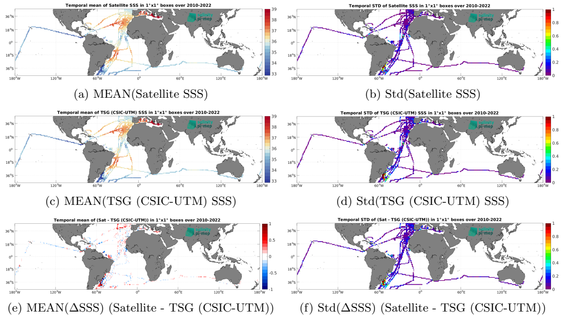
Figure 6: Temporal mean (left) and Std (right) of SSS from CCI SSS L4 Merged-OI v4.4 - 7-day running (ESA) (top), TSG (CSIC-UTM) (middle), and of \Delta SSS (Satellite - TSG (CSIC-UTM)). Only match-up pairs are used to generate these maps.
