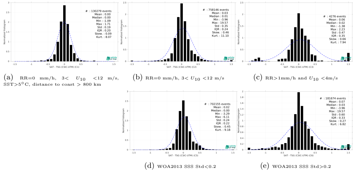
Figure 13: Normalized histogram of \Delta\text{SSS} (CCI SSS L4 Merged-OI v4.4 - 7-day running (ESA) - TSG (CSIC-UTM)) for 5 different subdatasets corresponding to: RR=0 mm/h, 3 < U_{10} < 12 m/s, SST>5°C, distance to coast > 800 km (a), RR=0 mm/h, 3 < U_{10} < 12 m/s (b), RR>1mm/h and U_{10} < 4 m/s (c), WOA2013 SSS Std<0.2 (d), WOA2013 SSS Std>0.2 (e).
