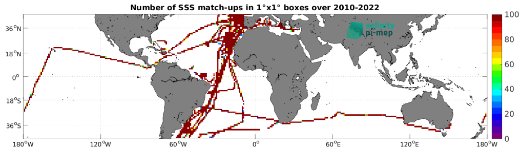
Figure 4: Number of SSS match-ups between TSG (CSIC-UTM) SSS and the CCI SSS L4 Merged-OI v4.4 - 7-day running (ESA) SSS product for the Mid-Low Latitudes 45N-45S Pi-MEP region over 1^\circ \times 1^\circ boxes and for the full satellite product period.
