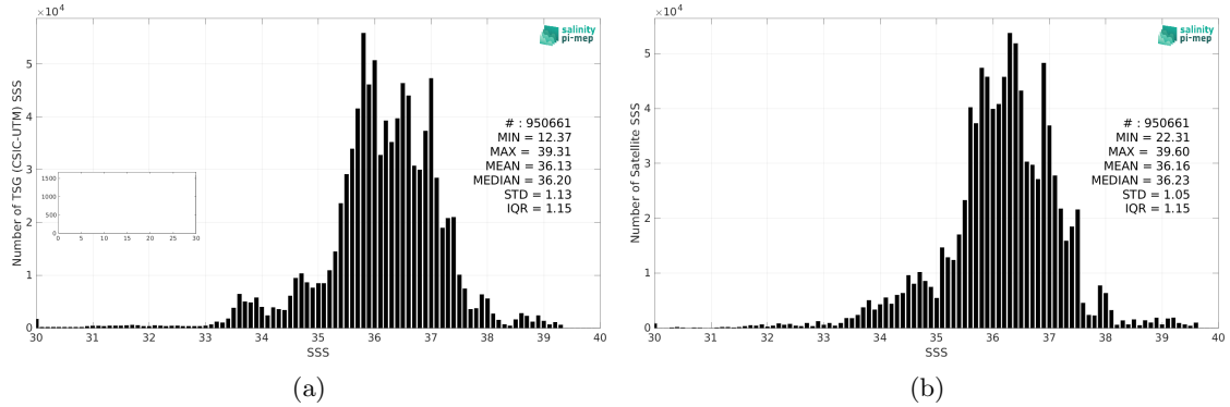
Figure 2: Histograms of SSS from TSG (CSIC-UTM) (a) and CCI SSS L4 Merged-OI v4.4 - 7-day running (ESA) (b) considering all match-up pairs per bins of 0.1 over the Mid-Low Latitudes 45N-45S Pi-MEP region and for the full satellite product period.
