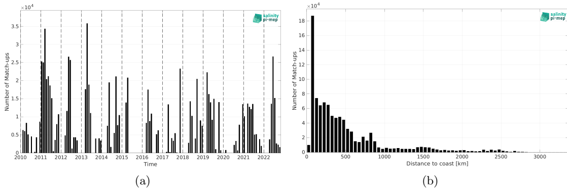
Figure 1: Number of match-ups between TSG (CSIC-UTM) and CCI SSS L4 Merged-OI v4.4 - 7-day running (ESA) SSS as a function of time (a) and as function of the distance to coast (b) over the Mid-Low Latitudes 45N-45S Pi-MEP region and for the full satellite product period.
