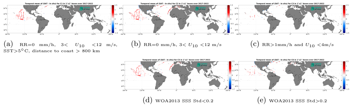
Figure 12: Temporal mean gridded over spatial boxes of size 1^\circ \times 1^\circ of \Delta SSS (CCI SSS L4 Merged-OI v4.4 - 7-day running (ESA) - Saildrone) for 5 different subdatasets corresponding to:RR=0 mm/h, 3 < U_{10} < 12 m/s, SST >5^\circ C, distance to coast > 800 km (a), RR=0 mm/h, 3 < U_{10} < 12 m/s (b), RR >1 mm/h and U_{10} < 4 m/s (c), WOA2013 SSS Std <0.2 (d), WOA2013 SSS Std >0.2 (e).
