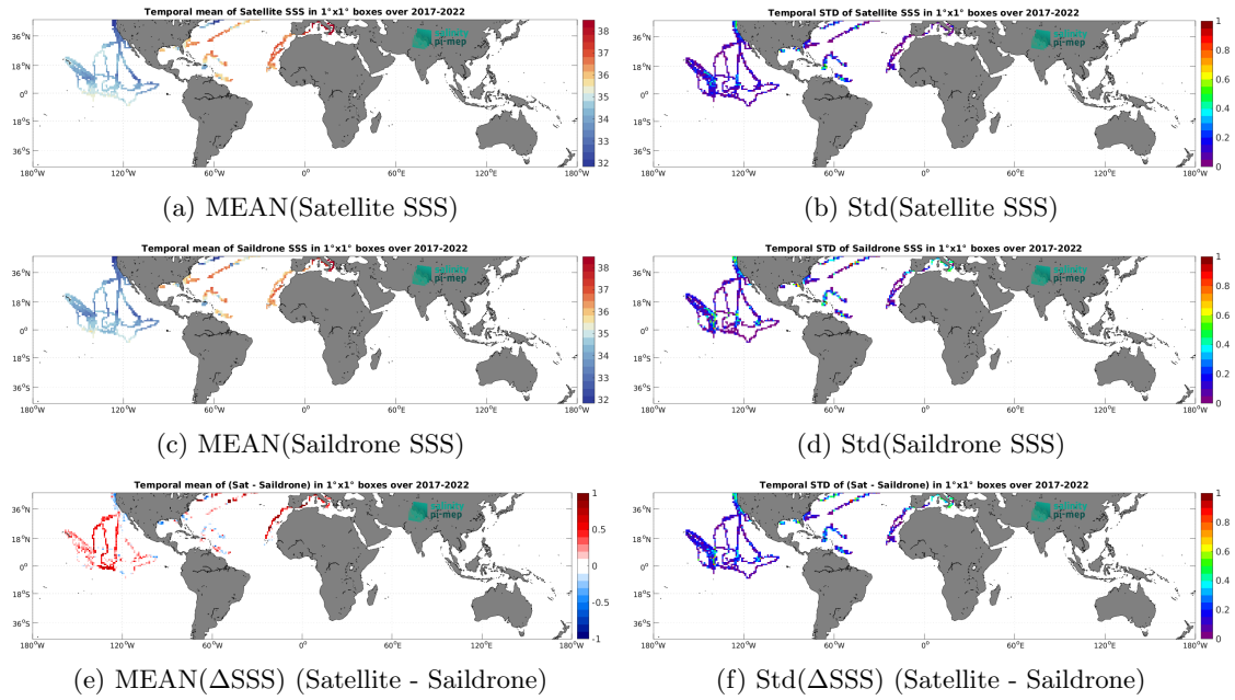
Figure 6: Temporal mean (left) and Std (right) of SSS from CCI SSS L4 Merged-OI v4.4 - 7-day running (ESA) (top), Saildrone (middle), and of \Delta SSS (Satellite - Saildrone). Only match-up pairs are used to generate these maps.
