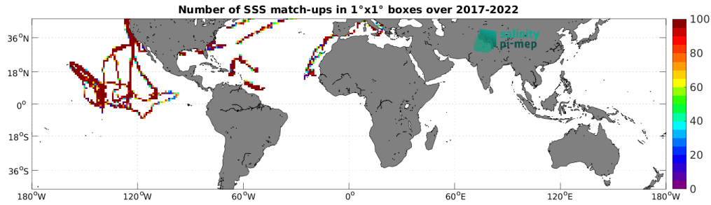
Figure 4: Number of SSS match-ups between Saildrone SSS and the CCI SSS L4 Merged-OI v4.4 - 7-day running (ESA) SSS product for the Mid-Low Latitudes 45N-45S Pi-MEP region over 1^\circ \times 1^\circ boxes and for the full satellite product period.
