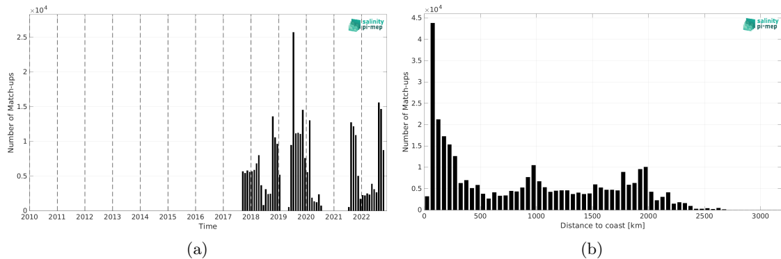
Figure 1: Number of match-ups between Saildrone and CCI SSS L4 Merged-OI v4.4 - 7-day running (ESA) SSS as a function of time (a) and as function of the distance to coast (b) over the Mid-Low Latitudes 45N-45S Pi-MEP region and for the full satellite product period.
