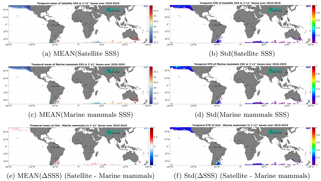
Figure 6: Temporal mean (left) and Std (right) of SSS from CCI SSS L4 Merged-OI v4.4 - 7-day running (ESA) (top), Marine mammals (middle), and of \Delta SSS (Satellite - Marine mammals). Only match-up pairs are used to generate these maps.
