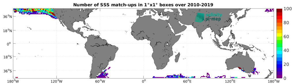
Figure 4: Number of SSS match-ups between Marine mammals SSS and the CCI SSS L4 Merged-OI v4.4 - 7-day running (ESA) SSS product for the Mid-Low Latitudes 45N-45S Pi-MEP region over 1^\circ \times 1^\circ boxes and for the full satellite product period.
