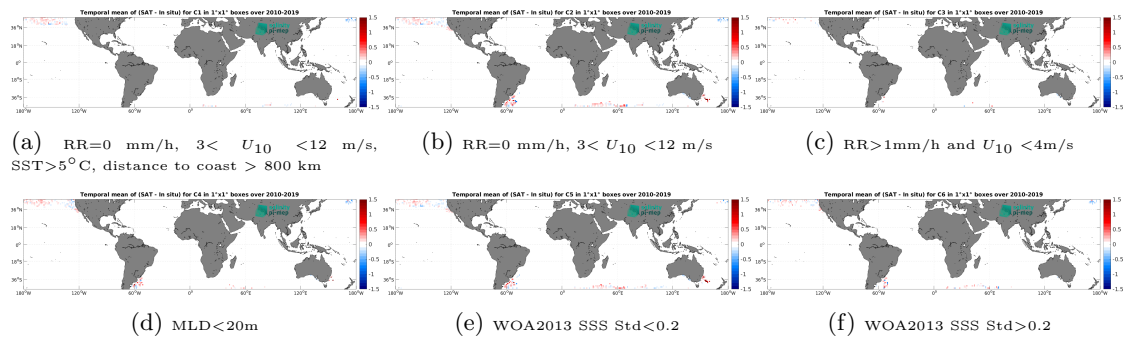
Figure 12: Temporal mean gridded over spatial boxes of size 1^\circ \times 1^\circ of \Delta SSS (CCI SSS L4 Merged-OI v4.4 - 7-day running (ESA) - Marine mammals) for 6 different subdatasets corresponding to:RR=0 mm/h, 3 < U_{10} < 12 m/s, SST >5^\circ C, distance to coast > 800 km (a), RR=0 mm/h, 3 < U_{10} < 12 m/s (b), RR >1 mm/h and U_{10} < 4 m/s (c),MLD <20 m (d),WOA2013 SSS Std <0.2 (e),WOA2013 SSS Std >0.2 (f).
