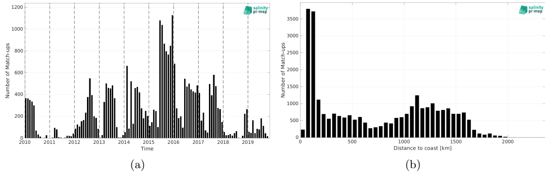
Figure 1: Number of match-ups between Marine mammals and CCI SSS L4 Merged-OI v4.4 - 7-day running (ESA) SSS as a function of time (a) and as function of the distance to coast (b) over the Mid-Low Latitudes 45N-45S Pi-MEP region and for the full satellite product period.
