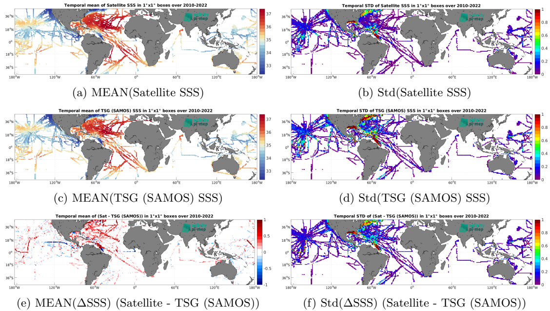
Figure 6: Temporal mean (left) and Std (right) of SSS from CCI SSS L4 Merged-OI v4.4 - 30-day running (ESA) (top), TSG (SAMOS) (middle), and of \Delta SSS (Satellite - TSG (SAMOS)). Only match-up pairs are used to generate these maps.
