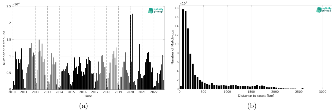
Figure 1: Number of match-ups between TSG (SAMOS) and CCI SSS L4 Merged-OI v4.4 - 30-day running (ESA) SSS as a function of time (a) and as function of the distance to coast (b) over the Mid-Low Latitudes 45N-45S Pi-MEP region and for the full satellite product period.
