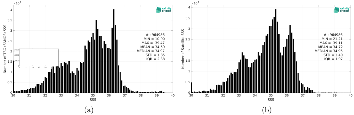
Figure 2: Histograms of SSS from TSG (SAMOS) (a) and CCI SSS L4 Merged-OI v4.4 - 30-day running (ESA) (b) considering all match-up pairs per bins of 0.1 over the Mid-Low Latitudes 45N-45S Pi-MEP region and for the full satellite product period.
