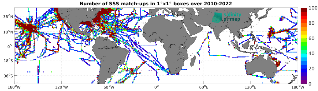
Figure 4: Number of SSS match-ups between TSG (SAMOS) SSS and the CCI SSS L4 Merged-OI v4.4 - 30-day running (ESA) SSS product for the Mid-Low Latitudes 45N-45S Pi-MEP region over 1^\circ \times 1^\circ boxes and for the full satellite product period.
