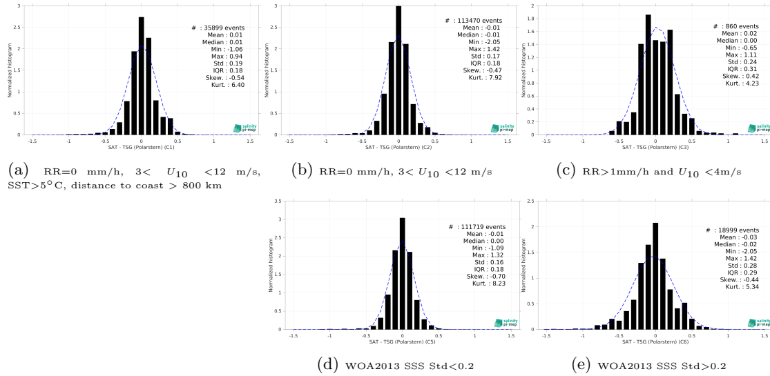
Figure 13: Normalized histogram of \Delta\text{SSS} (CCI SSS L4 Merged-OI v4.4 - 30-day running (ESA) - TSG (Polarstern)) for 5 different subdatasets corresponding to: RR=0 mm/h, 3 < U_{10} < 12 m/s, SST>5°C, distance to coast > 800 km (a), RR=0 mm/h, 3 < U_{10} < 12 m/s (b), RR>1mm/h and U_{10} < 4 m/s (c), WOA2013 SSS Std<0.2 (d), WOA2013 SSS Std>0.2 (e).
