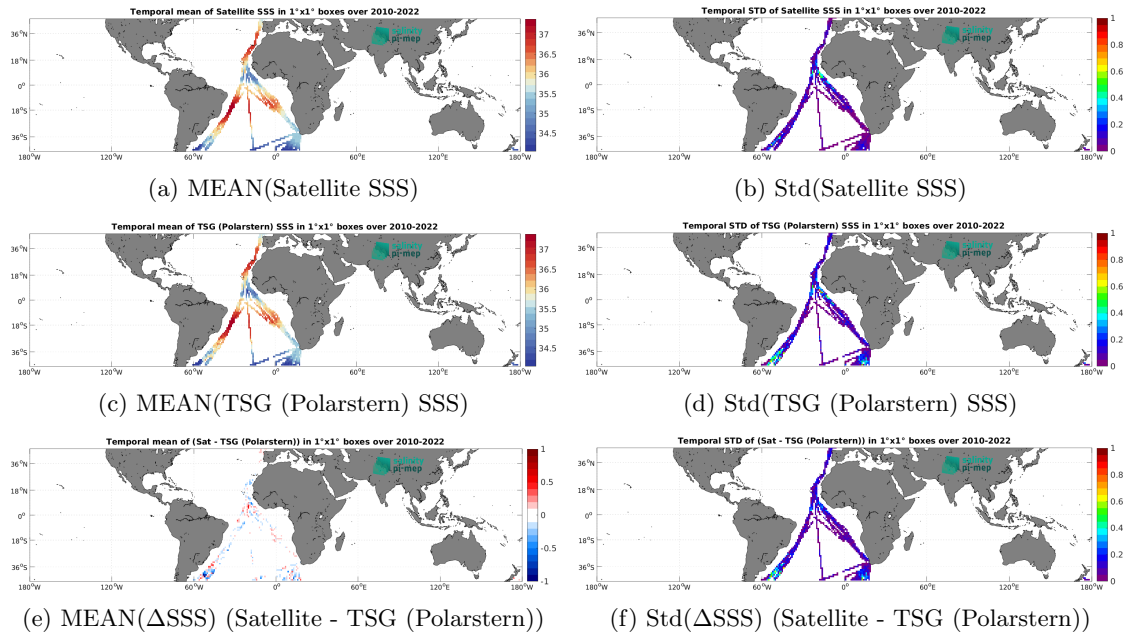
Figure 6: Temporal mean (left) and Std (right) of SSS from CCI SSS L4 Merged-OI v4.4 - 30-day running (ESA) (top), TSG (Polarstern) (middle), and of \Delta SSS (Satellite - TSG (Polarstern)). Only match-up pairs are used to generate these maps.
