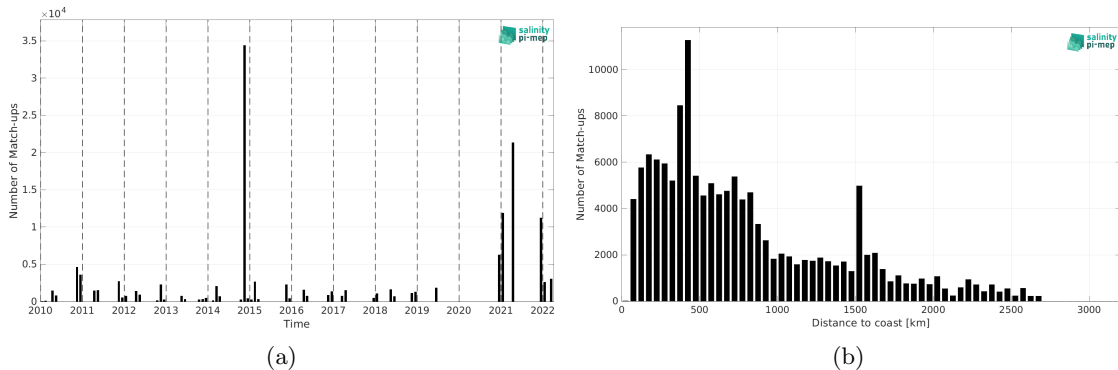
Figure 1: Number of match-ups between TSG (Polarstern) and CCI SSS L4 Merged-OI v4.4 - 30-day running (ESA) SSS as a function of time (a) and as function of the distance to coast (b) over the Mid-Low Latitudes 45N-45S Pi-MEP region and for the full satellite product period.
