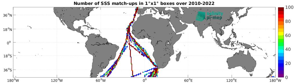
Figure 4: Number of SSS match-ups between TSG (Polarstern) SSS and the CCI SSS L4 Merged-OI v4.4 - 30-day running (ESA) SSS product for the Mid-Low Latitudes 45N-45S Pi-MEP region over 1^\circ \times 1^\circ boxes and for the full satellite product period.
