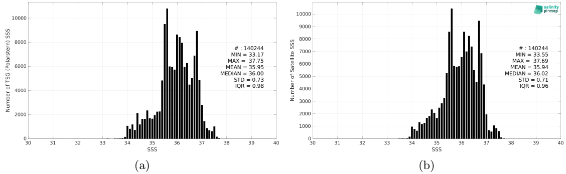
Figure 2: Histograms of SSS from TSG (Polarstern) (a) and CCI SSS L4 Merged-OI v4.4 - 30-day running (ESA) (b) considering all match-up pairs per bins of 0.1 over the Mid-Low Latitudes 45N-45S Pi-MEP region and for the full satellite product period.
