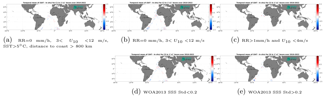
Figure 12: Temporal mean gridded over spatial boxes of size 1^\circ \times 1^\circ of \Delta SSS (CCI SSS L4 Merged-OI v4.4 - 30-day running (ESA) - TSG (Polarstern)) for 5 different subdatasets corresponding to:RR=0 mm/h, 3 < U_{10} < 12 m/s, SST >5^\circ C, distance to coast > 800 km (a), RR=0 mm/h, 3 < U_{10} < 12 m/s (b), RR >1 mm/h and U_{10} < 4 m/s (c), WOA2013 SSS Std <0.2 (d), WOA2013 SSS Std >0.2 (e).
