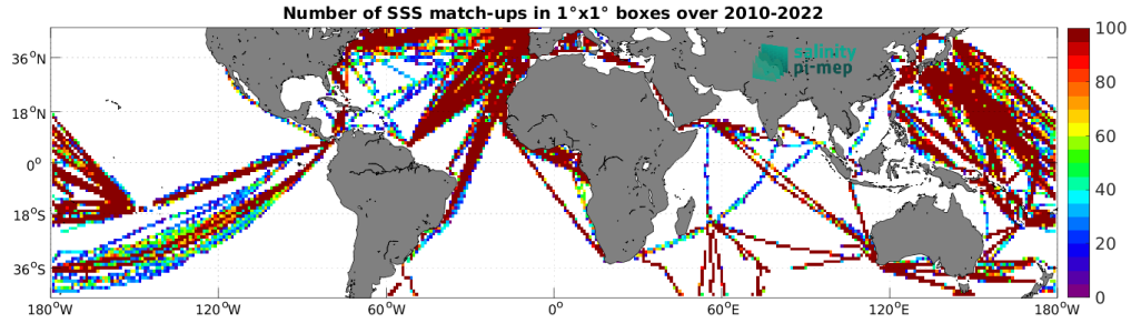
Figure 4: Number of SSS match-ups between TSG (LEGOS-DM) SSS and the CCI SSS L4 Merged-OI v4.4 - 30-day running (ESA) SSS product for the Mid-Low Latitudes 45N-45S Pi-MEP region over 1^\circ \times 1^\circ boxes and for the full satellite product period.
