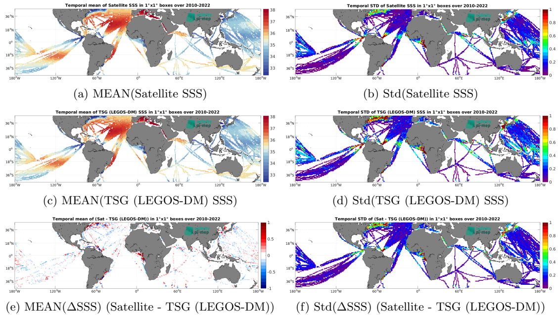
Figure 6: Temporal mean (left) and Std (right) of SSS from CCI SSS L4 Merged-OI v4.4 - 30-day running (ESA) (top), TSG (LEGOS-DM) (middle), and of \Delta SSS (Satellite - TSG (LEGOS-DM)). Only match-up pairs are used to generate these maps.
