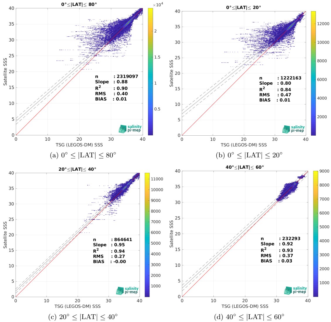
Figure 9: Contour maps of the concentration of CCI SSS L4 Merged-OI v4.4 - 30-day running (ESA) SSS (y-axis) versus TSG (LEGOS-DM) SSS (x-axis) at match-up pairs for different latitude bands. For each plot, the red line shows x=y . The black thin and dashed lines indicate a linear fit through the data cloud and the \pm 95\% confidence levels, respectively. The number of match-up pairs n , the slope and R^2 coefficient of the linear fit, the root mean square (RMS) and the mean bias between satellite and in situ data are indicated for each latitude band in each plot.
