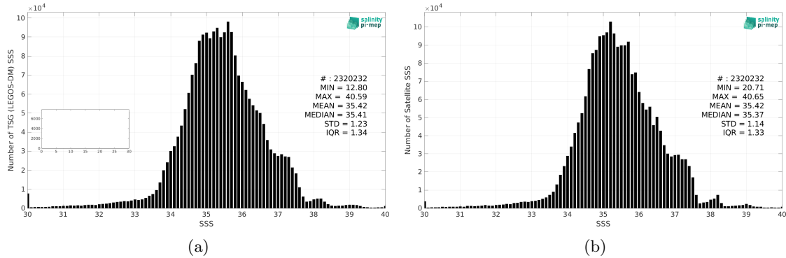
Figure 2: Histograms of SSS from TSG (LEGOS-DM) (a) and CCI SSS L4 Merged-OI v4.4 - 30-day running (ESA) (b) considering all match-up pairs per bins of 0.1 over the Mid-Low Latitudes 45N-45S Pi-MEP region and for the full satellite product period.
