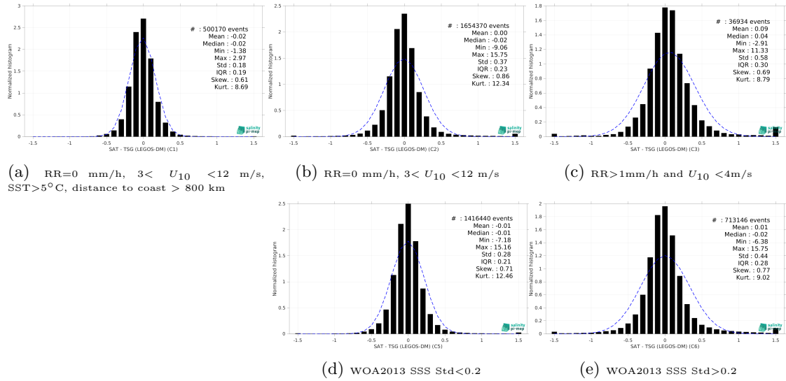
Figure 13: Normalized histogram of \Delta SSS (CCI SSS L4 Merged-OI v4.4 - 30-day running (ESA) - TSG (LEGOS-DM)) for 5 different subdatasets corresponding to: RR=0 mm/h, 3 < U_{10} < 12 m/s, SST>5°C, distance to coast > 800 km (a), RR=0 mm/h, 3 < U_{10} < 12 m/s (b), RR>1mm/h and U_{10} < 4 m/s (c), WOA2013 SSS Std<0.2 (d), WOA2013 SSS Std>0.2 (e).
