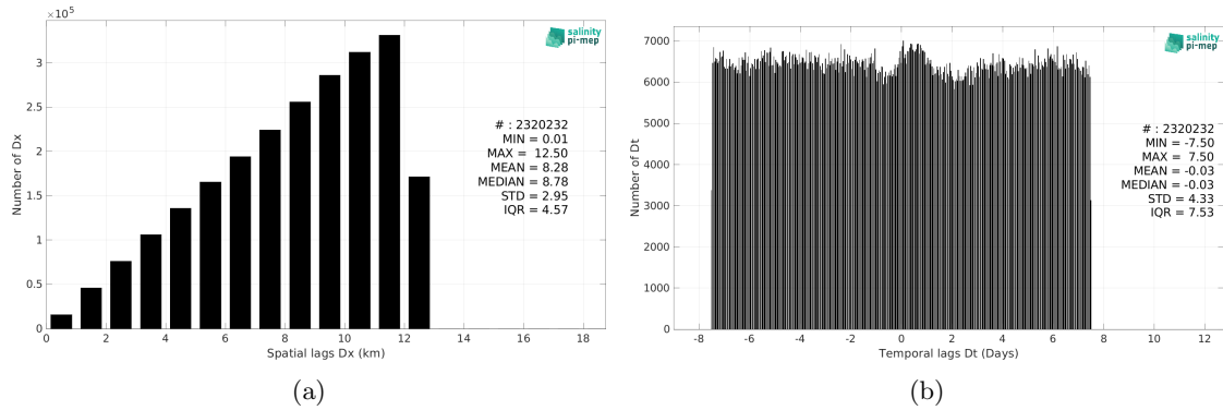
Figure 5: Histograms of the spatial (a) and temporal (b) lags between the location/time of the TSG (LEGOS-DM) measurement and the date of the corresponding CCI SSS L4 Merged-OI v4.4 - 30-day running (ESA) SSS pixel.
