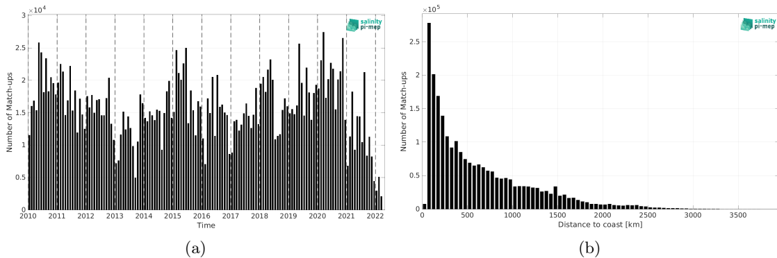
Figure 1: Number of match-ups between TSG (LEGOS-DM) and CCI SSS L4 Merged-OI v4.4 - 30-day running (ESA) SSS as a function of time (a) and as function of the distance to coast (b) over the Mid-Low Latitudes 45N-45S Pi-MEP region and for the full satellite product period.
