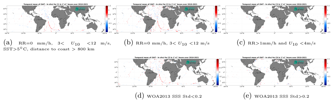
Figure 12: Temporal mean gridded over spatial boxes of size 1^\circ \times 1^\circ of \Delta\text{SSS} (CCI SSS L4 Merged-OI v4.4 - 30-day running (ESA) - TSG (GOSUD-Sailing-ship)) for 5 different subdatasets corresponding to: RR=0 mm/h, 3 < U_{10} < 12 m/s, SST > 5°C, distance to coast > 800 km (a), RR=0 mm/h, 3 < U_{10} < 12 m/s (b), RR > 1mm/h and U_{10} < 4 m/s (c), WOA2013 SSS Std < 0.2 (d), WOA2013 SSS Std > 0.2 (e).
