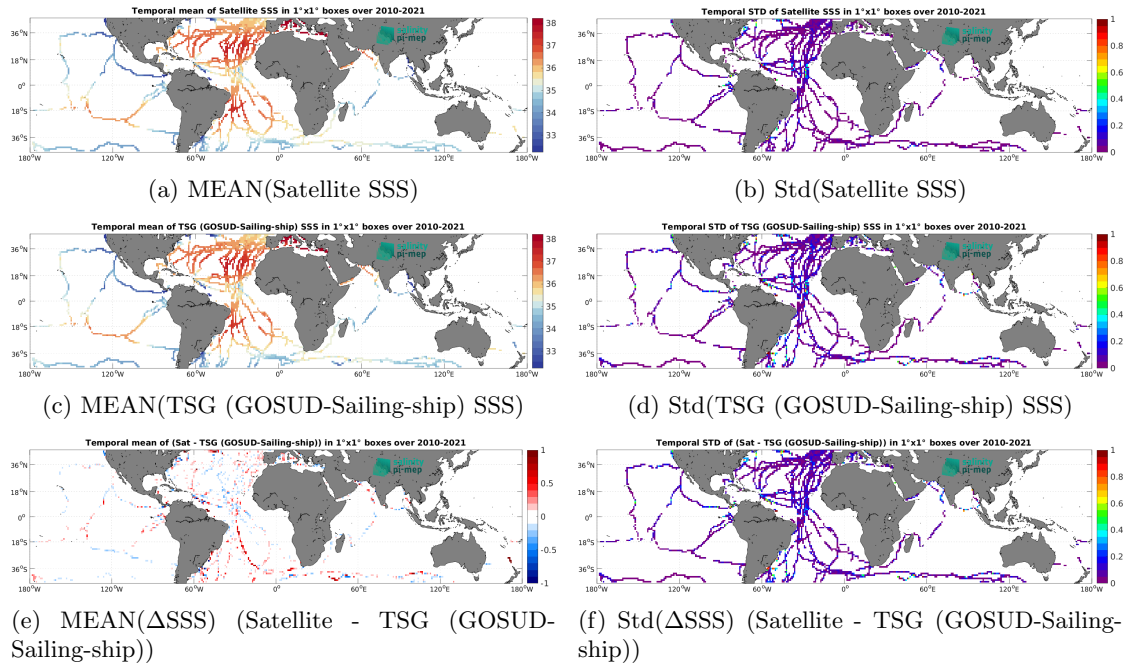
Figure 6: Temporal mean (left) and Std (right) of SSS from CCI SSS L4 Merged-OI v4.4 - 30-day running (ESA) (top), TSG (GOSUD-Sailing-ship) (middle), and of \Delta SSS (Satellite - TSG (GOSUD-Sailing-ship)). Only match-up pairs are used to generate these maps.
