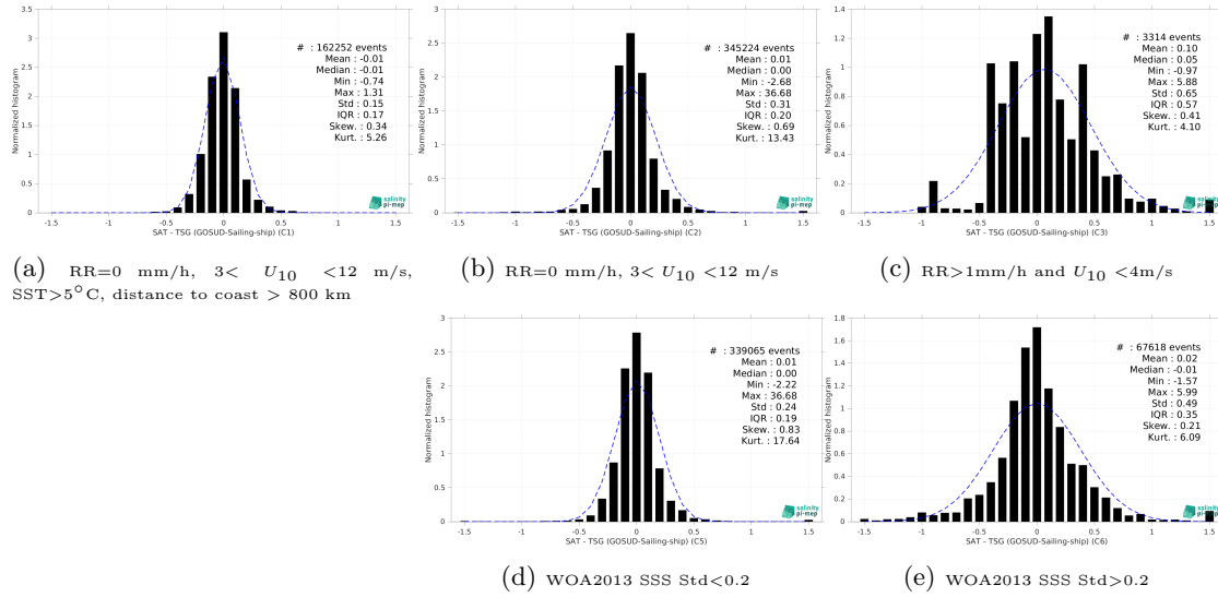
Figure 13: Normalized histogram of \Delta\text{SSS} (CCI SSS L4 Merged-OI v4.4 - 30-day running (ESA) - TSG (GOSUD-Sailing-ship)) for 5 different subdatasets corresponding to: RR=0 mm/h, 3 < U_{10} < 12 m/s, SST>5°C, distance to coast > 800 km (a), RR=0 mm/h, 3 < U_{10} < 12 m/s (b), RR>1mm/h and U_{10} < 4 m/s (c), WOA2013 SSS Std<0.2 (d), WOA2013 SSS Std>0.2 (e).
