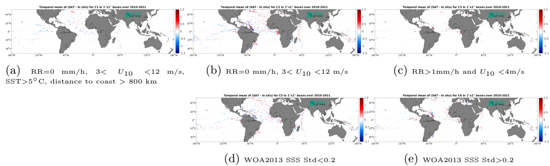
Figure 12: Temporal mean gridded over spatial boxes of size 1^\circ \times 1^\circ of \Delta SSS (CCI SSS L4 Merged-OI v4.4 - 30-day running (ESA) - TSG (GOSUD-Research-vessel)) for 5 different subdatasets corresponding to:RR=0 mm/h, 3 < U_{10} < 12 m/s, SST > 5^\circ\text{C} , distance to coast > 800 km (a), RR=0 mm/h, 3 < U_{10} < 12 m/s (b), RR > 1 mm/h and U_{10} < 4 m/s (c), WOA2013 SSS Std < 0.2 (d), WOA2013 SSS Std > 0.2 (e).
