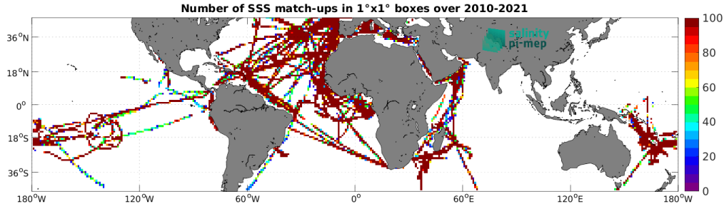
Figure 4: Number of SSS match-ups between TSG (GOSUD-Research-vessel) SSS and the CCI SSS L4 Merged-OI v4.4 - 30-day running (ESA) SSS product for the Mid-Low Latitudes 45N-45S Pi-MEP region over 1^\circ \times 1^\circ boxes and for the full satellite product period.
