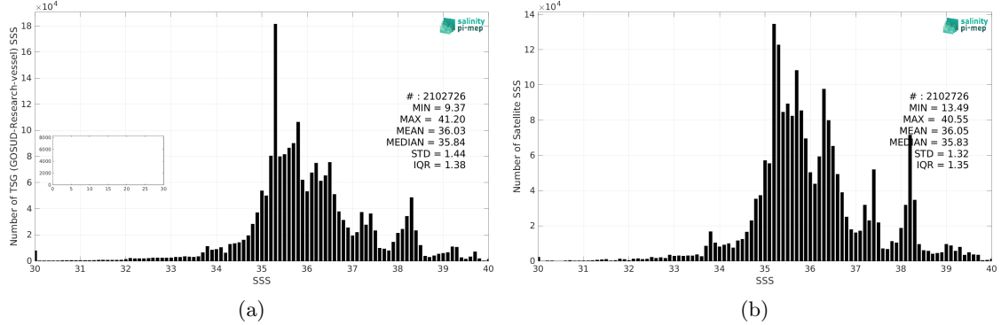
Figure 2: Histograms of SSS from TSG (GOSUD-Research-vessel) (a) and CCI SSS L4 Merged-OI v4.4 - 30-day running (ESA) (b) considering all match-up pairs per bins of 0.1 over the Mid-Low Latitudes 45N-45S Pi-MEP region and for the full satellite product period.
