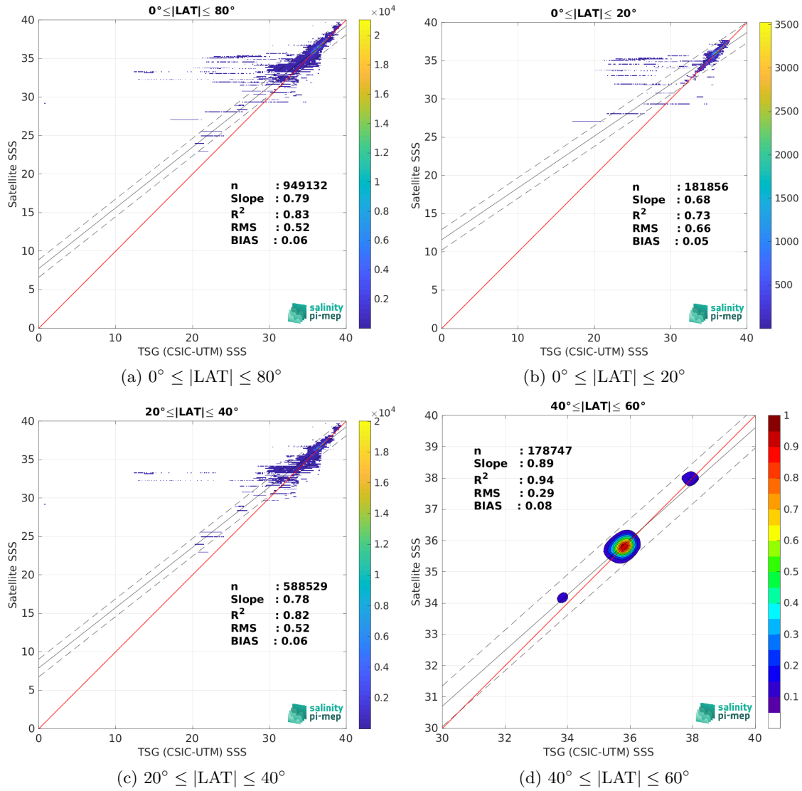
Figure 9: Contour maps of the concentration of CCI SSS L4 Merged-OI v4.4 - 30-day running (ESA) SSS (y-axis) versus TSG (CSIC-UTM) SSS (x-axis) at match-up pairs for different latitude bands. For each plot, the red line shows x=y . The black thin and dashed lines indicate a linear fit through the data cloud and the \pm 95\% confidence levels, respectively. The number match-up pairs n , the slope and R^2 coefficient of the linear fit, the root mean square (RMS) and the mean bias between satellite and in situ data are indicated for each latitude band in each plots.
