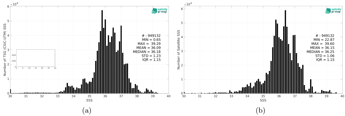
Figure 2: Histograms of SSS from TSG (CSIC-UTM) (a) and CCI SSS L4 Merged-OI v4.4 - 30-day running (ESA) (b) considering all match-up pairs per bins of 0.1 over the Mid-Low Latitudes 45N-45S Pi-MEP region and for the full satellite product period.
