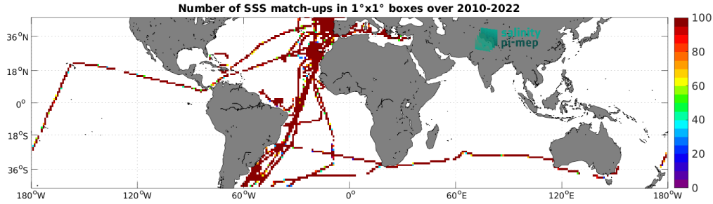
Figure 4: Number of SSS match-ups between TSG (CSIC-UTM) SSS and the CCI SSS L4 Merged-OI v4.4 - 30-day running (ESA) SSS product for the Mid-Low Latitudes 45N-45S Pi-MEP region over 1^\circ \times 1^\circ boxes and for the full satellite product period.
