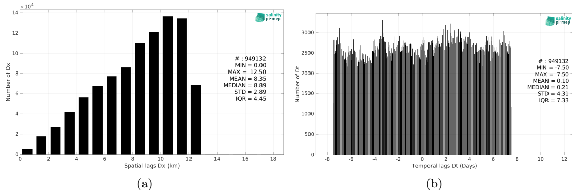
Figure 5: Histograms of the spatial (a) and temporal (b) lags between the location/time of the TSG (CSIC-UTM) measurement and the date of the corresponding CCI SSS L4 Merged-OI v4.4 - 30-day running (ESA) SSS pixel.
