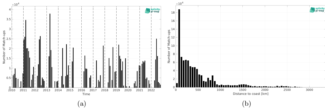
Figure 1: Number of match-ups between TSG (CSIC-UTM) and CCI SSS L4 Merged-OI v4.4 - 30-day running (ESA) SSS as a function of time (a) and as function of the distance to coast (b) over the Mid-Low Latitudes 45N-45S Pi-MEP region and for the full satellite product period.
