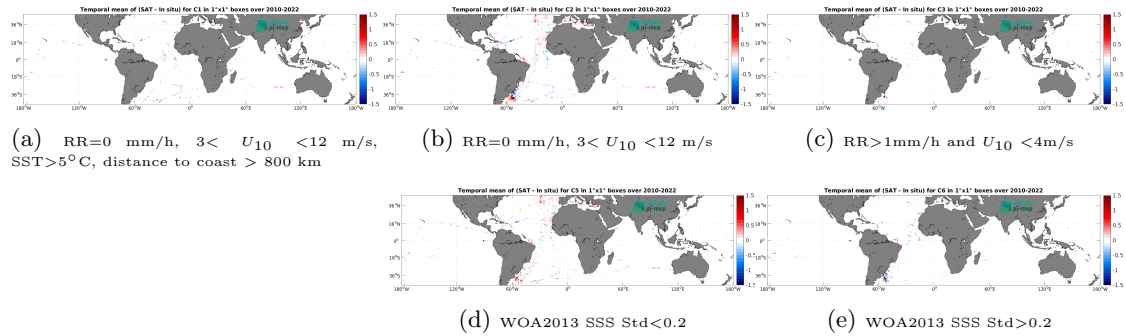
Figure 12: Temporal mean gridded over spatial boxes of size 1^\circ \times 1^\circ of \Delta SSS (CCI SSS L4 Merged-OI v4.4 - 30-day running (ESA) - TSG (CSIC-UTM)) for 5 different subdatasets corresponding to:RR=0 mm/h, 3 < U_{10} < 12 m/s, SST >5^\circ\text{C} , distance to coast > 800 km (a), RR=0 mm/h, 3 < U_{10} < 12 m/s (b), RR >1 mm/h and U_{10} < 4 m/s (c), WOA2013 SSS Std <0.2 (d), WOA2013 SSS Std >0.2 (e).
