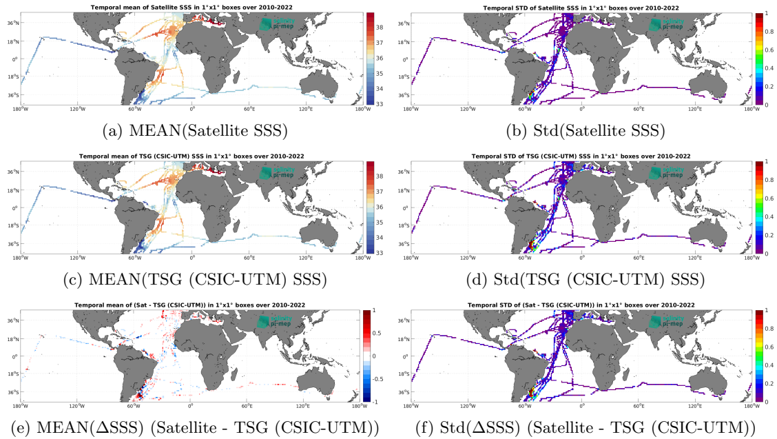
Figure 6: Temporal mean (left) and Std (right) of SSS from CCI SSS L4 Merged-OI v4.4 - 30-day running (ESA) (top), TSG (CSIC-UTM) (middle), and of \Delta SSS (Satellite - TSG (CSIC-UTM)). Only match-up pairs are used to generate these maps.
