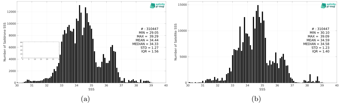
Figure 2: Histograms of SSS from Saildrone (a) and CCI SSS L4 Merged-OI v4.4 - 30-day running (ESA) (b) considering all match-up pairs per bins of 0.1 over the Mid-Low Latitudes 45N-45S Pi-MEP region and for the full satellite product period.
