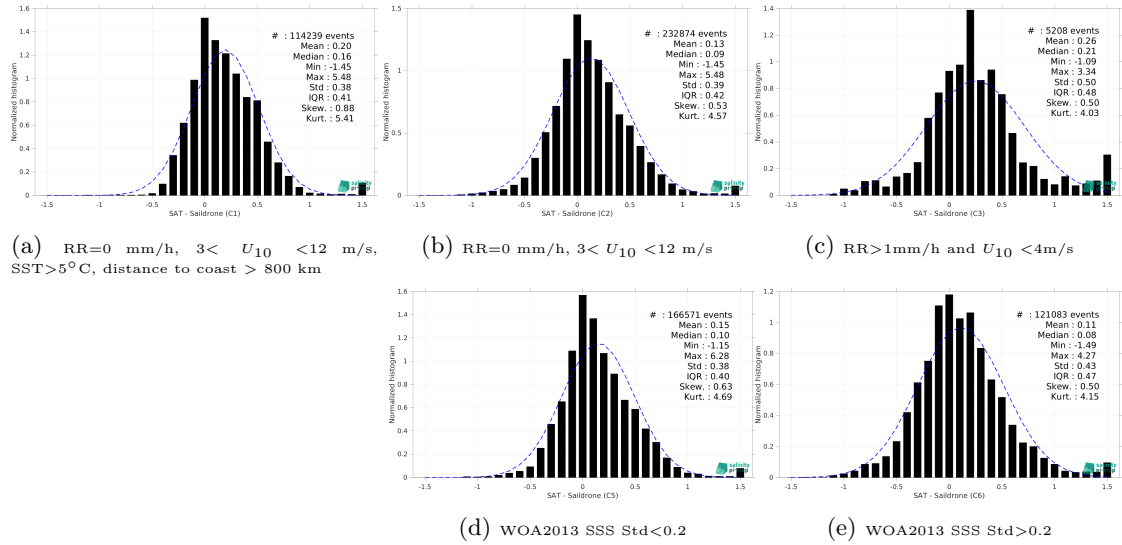
Figure 13: Normalized histogram of \Delta SSS (CCI SSS L4 Merged-OI v4.4 - 30-day running (ESA) - Sailldrone) for 5 different subdatasets corresponding to: RR=0 mm/h, 3 < U_{10} < 12 m/s, SST>5°C, distance to coast > 800 km (a), RR=0 mm/h, 3 < U_{10} < 12 m/s (b), RR>1mm/h and U_{10} < 4 m/s (c), WOA2013 SSS Std<0.2 (d), WOA2013 SSS Std>0.2 (e).
