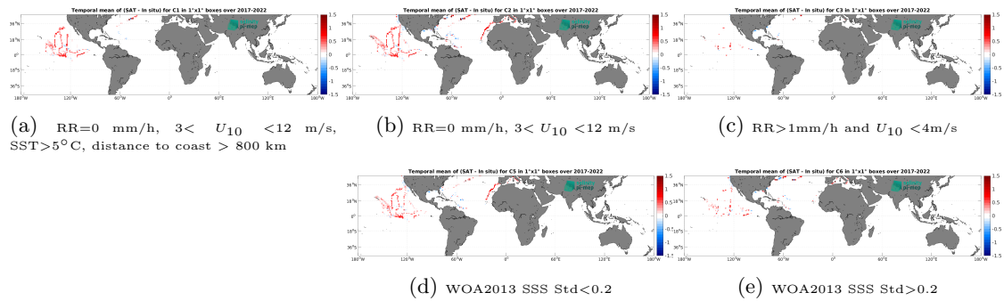
Figure 12: Temporal mean gridded over spatial boxes of size 1^\circ \times 1^\circ of \Delta SSS (CCI SSS L4 Merged-OI v4.4 - 30-day running (ESA) - Saildrone) for 5 different subdatasets corresponding to:RR=0 mm/h, 3 < U_{10} < 12 m/s, SST >5^\circ C, distance to coast > 800 km (a), RR=0 mm/h, 3 < U_{10} < 12 m/s (b), RR >1 mm/h and U_{10} < 4 m/s (c), WOA2013 SSS Std <0.2 (d), WOA2013 SSS Std >0.2 (e).
