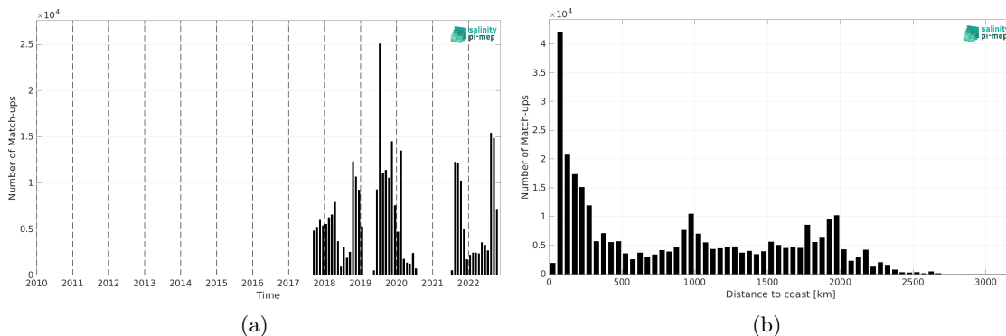
Figure 1: Number of match-ups between Saildrone and CCI SSS L4 Merged-OI v4.4 - 30-day running (ESA) SSS as a function of time (a) and as function of the distance to coast (b) over the Mid-Low Latitudes 45N-45S Pi-MEP region and for the full satellite product period.
