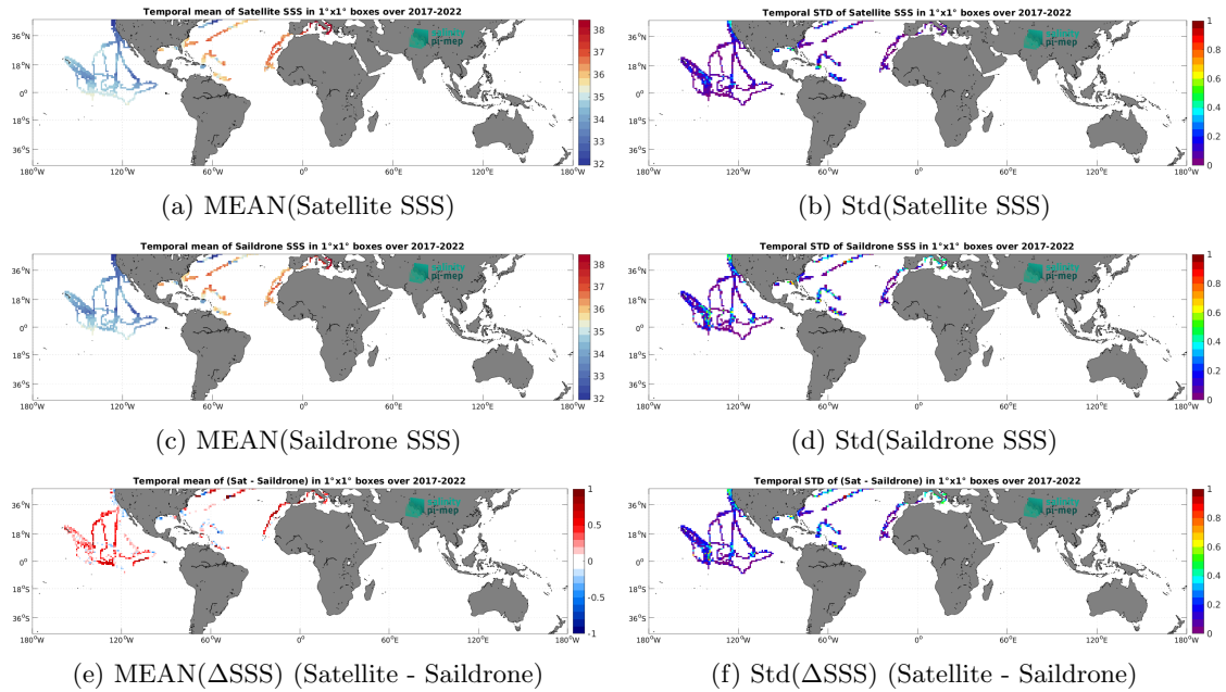
Figure 6: Temporal mean (left) and Std (right) of SSS from CCI SSS L4 Merged-OI v4.4 - 30-day running (ESA) (top), Saildrone (middle), and of \Delta SSS (Satellite - Saildrone). Only match-up pairs are used to generate these maps.
