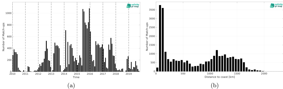
Figure 1: Number of match-ups between Marine mammals and CCI SSS L4 Merged-OI v4.4 - 30-day running (ESA) SSS as a function of time (a) and as function of the distance to coast (b) over the Mid-Low Latitudes 45N-45S Pi-MEP region and for the full satellite product period.
