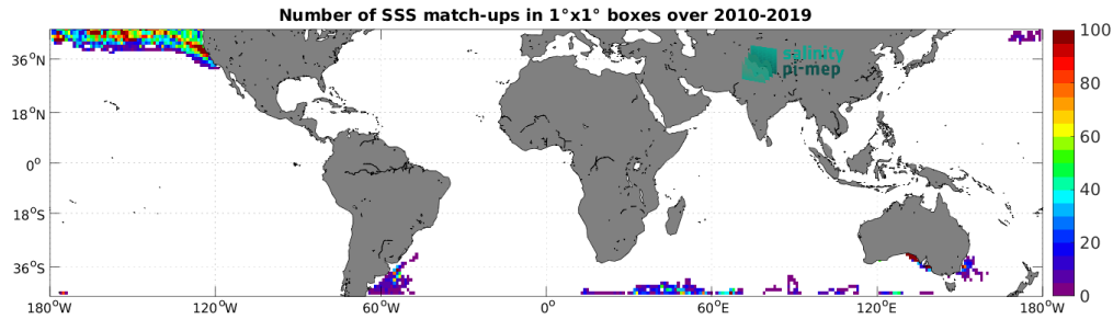
Figure 4: Number of SSS match-ups between Marine mammals SSS and the CCI SSS L4 Merged-OI v4.4 - 30-day running (ESA) SSS product for the Mid-Low Latitudes 45N-45S Pi-MEP region over 1^\circ \times 1^\circ boxes and for the full satellite product period.
