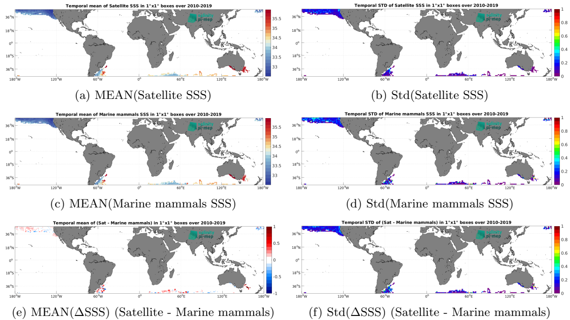
Figure 6: Temporal mean (left) and Std (right) of SSS from CCI SSS L4 Merged-OI v4.4 - 30-day running (ESA) (top), Marine mammals (middle), and of \Delta SSS (Satellite - Marine mammals). Only match-up pairs are used to generate these maps.
