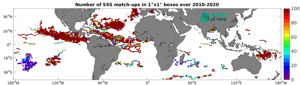
Figure 3: Number of SSS match-ups between Surface drifters SSS and the CCI SSS L4 Merged-OI v4.4 - 30-day running (ESA) SSS product for the Mid-Low Latitudes 45N-45S Pi-MEP region over 1^\circ \times 1^\circ boxes and for the full satellite product period.
