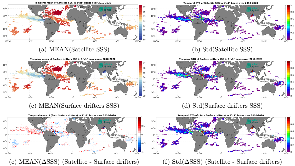
Figure 5: Temporal mean (left) and Std (right) of SSS from CCI SSS L4 Merged-OI v4.4 - 30-day running (ESA) (top), Surface drifters (middle), and of \Delta SSS (Satellite - Surface drifters). Only match-up pairs are used to generate these maps.
