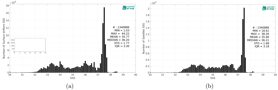
Figure 2: Histograms of SSS from Surface drifters (a) and CCI SSS L4 Merged-OI v4.4 - 30-day running (ESA) (b) considering all match-up pairs per bins of 0.1 over the Mid-Low Latitudes 45N-45S Pi-MEP region and for the full satellite product period.
