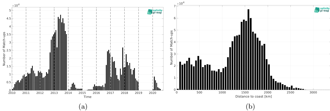
Figure 1: Number of match-ups between Surface drifters and CCI SSS L4 Merged-OI v4.4 - 30-day running (ESA) SSS as a function of time (a) and as function of the distance to coast (b) over the Mid-Low Latitudes 45N-45S Pi-MEP region and for the full satellite product period.
