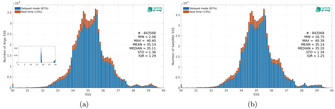
Figure 2: Histograms of SSS from Argo (a) and CCI SSS L4 Merged-OI v4.4 - 30-day running (ESA) (b) considering all match-up pairs per bins of 0.1 over the Mid-Low Latitudes 45N-45S Pi-MEP region and for the full satellite product period.
