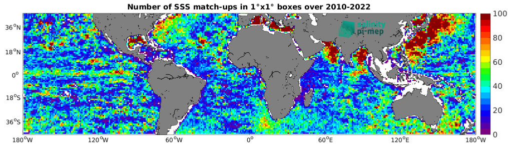
Figure 4: Number of SSS match-ups between Argo SSS and the CCI SSS L4 Merged-OI v4.4 - 30-day running (ESA) SSS product for the Mid-Low Latitudes 45N-45S Pi-MEP region over 1^\circ \times 1^\circ boxes and for the full satellite product period.
