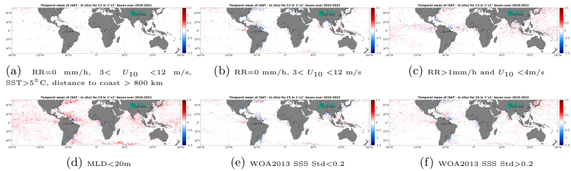
Figure 12: Temporal mean gridded over spatial boxes of size 1^\circ \times 1^\circ of \Delta SSS (CCI SSS L4 Merged-OI v4.4 - 30-day running (ESA) - Argo) for 6 different subdatasets corresponding to:RR=0 mm/h, 3 < U_{10} < 12 m/s, SST >5^\circ C, distance to coast > 800 km (a), RR=0 mm/h, 3 < U_{10} < 12 m/s (b), RR >1 mm/h and U_{10} < 4 m/s (c),MLD <20 m (d),WOA2013 SSS Std <0.2 (e),WOA2013 SSS Std >0.2 (f).
