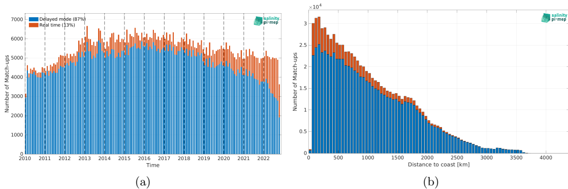
Figure 1: Number of match-ups between Argo and CCI SSS L4 Merged-OI v4.4 - 30-day running (ESA) SSS as a function of time (a) and as function of the distance to coast (b) over the Mid-Low Latitudes 45N-45S Pi-MEP region and for the full satellite product period.
