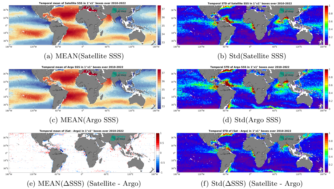
Figure 6: Temporal mean (left) and Std (right) of SSS from CCI SSS L4 Merged-OI v4.4 - 30-day running (ESA) (top), Argo (middle), and of \Delta SSS (Satellite - Argo). Only match-up pairs are used to generate these maps.
