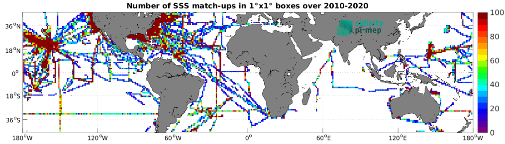
Figure 4: Number of SSS match-ups between TSG (SAMOS) SSS and the CCI SSS L4 Merged-OI v3.2 - 7-day running (ESA) SSS product for the Mid-Low Latitudes 45N-45S Pi-MEP region over 1^\circ \times 1^\circ boxes and for the full satellite product period.
