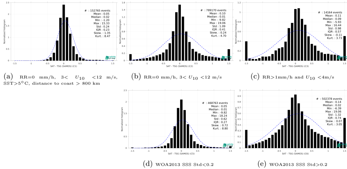
Figure 13: Normalized histogram of \Delta\text{SSS} (CCI SSS L4 Merged-OI v3.2 - 7-day running (ESA) - TSG (SAMOS)) for 5 different subdatasets corresponding to: RR=0 mm/h, 3 < U_{10} < 12 m/s, SST>5°C, distance to coast > 800 km (a), RR=0 mm/h, 3 < U_{10} < 12 m/s (b), RR>1mm/h and U_{10} < 4 m/s (c), WOA2013 SSS Std<0.2 (d), WOA2013 SSS Std>0.2 (e).
