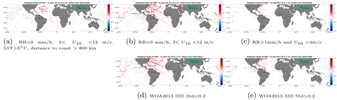
Figure 12: Temporal mean gridded over spatial boxes of size 1^\circ \times 1^\circ of \Delta SSS (CCI SSS L4 Merged-OI v3.2 - 7-day running (ESA) - TSG (SAMOS)) for 5 different subdatasets corresponding to:RR=0 mm/h, 3 < U_{10} < 12 m/s, SST >5^\circ\text{C} , distance to coast > 800 km (a), RR=0 mm/h, 3 < U_{10} < 12 m/s (b), RR >1 mm/h and U_{10} < 4 m/s (c), WOA2013 SSS Std <0.2 (d), WOA2013 SSS Std >0.2 (e).
