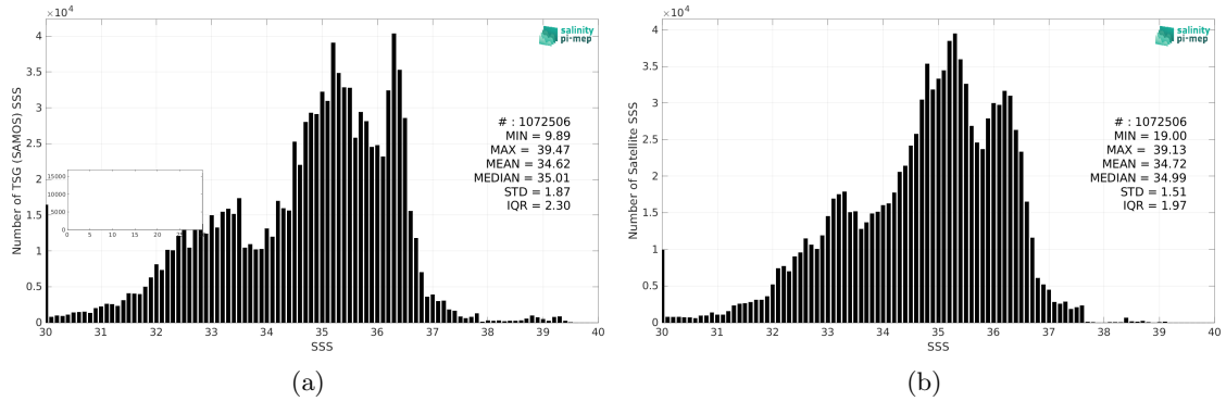
Figure 2: Histograms of SSS from TSG (SAMOS) (a) and CCI SSS L4 Merged-OI v3.2 - 7-day running (ESA) (b) considering all match-up pairs per bins of 0.1 over the Mid-Low Latitudes 45N-45S Pi-MEP region and for the full satellite product period.
