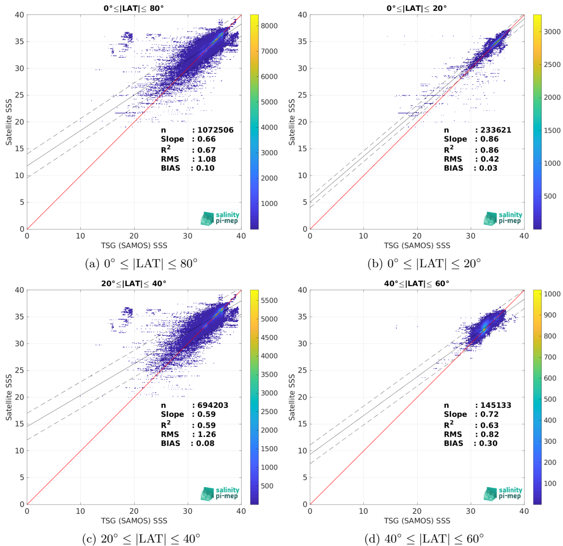
Figure 9: Contour maps of the concentration of CCI SSS L4 Merged-OI v3.2 - 7-day running (ESA) SSS (y-axis) versus TSG (SAMOS) SSS (x-axis) at match-up pairs for different latitude bands. For each plot, the red line shows x=y . The black thin and dashed lines indicate a linear fit through the data cloud and the \pm 95\% confidence levels, respectively. The number match-up pairs n , the slope and R^2 coefficient of the linear fit, the root mean square (RMS) and the mean bias between satellite and in situ data are indicated for each latitude band in each plots.
