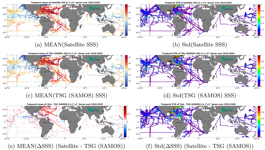
Figure 6: Temporal mean (left) and Std (right) of SSS from CCI SSS L4 Merged-OI v3.2 - 7-day running (ESA) (top), TSG (SAMOS) (middle), and of \Delta SSS (Satellite - TSG (SAMOS)). Only match-up pairs are used to generate these maps.
