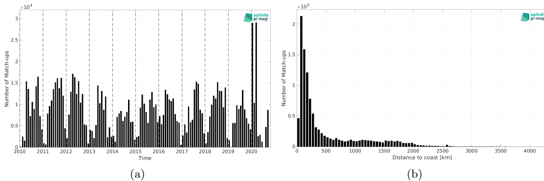
Figure 1: Number of match-ups between TSG (SAMOS) and CCI SSS L4 Merged-OI v3.2 - 7-day running (ESA) SSS as a function of time (a) and as function of the distance to coast (b) over the Mid-Low Latitudes 45N-45S Pi-MEP region and for the full satellite product period.
