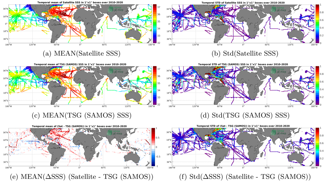
Figure 6: Temporal mean (left) and Std (right) of SSS from CCI SSS L4 Merged-OI v3.2 - 7-day running (ESA) (top), TSG (SAMOS) (middle), and of \Delta SSS (Satellite - TSG (SAMOS)). Only match-up pairs are used to generate these maps.
