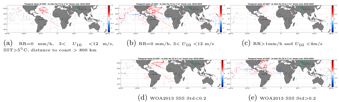
Figure 12: Temporal mean gridded over spatial boxes of size 1°x1° of \Delta SSS (CCI SSS L4 Merged-OI v3.2 - 7-day running (ESA) - TSG (SAMOS)) for 5 different subdatasets corresponding to:RR=0 mm/h, 3 < U_{10} < 12 m/s, SST>5°C, distance to coast > 800 km (a), RR=0 mm/h, 3 < U_{10} < 12 m/s (b), RR>1mm/h and U_{10} < 4 m/s (c), WOA2013 SSS Std<0.2 (d), WOA2013 SSS Std>0.2 (e).
