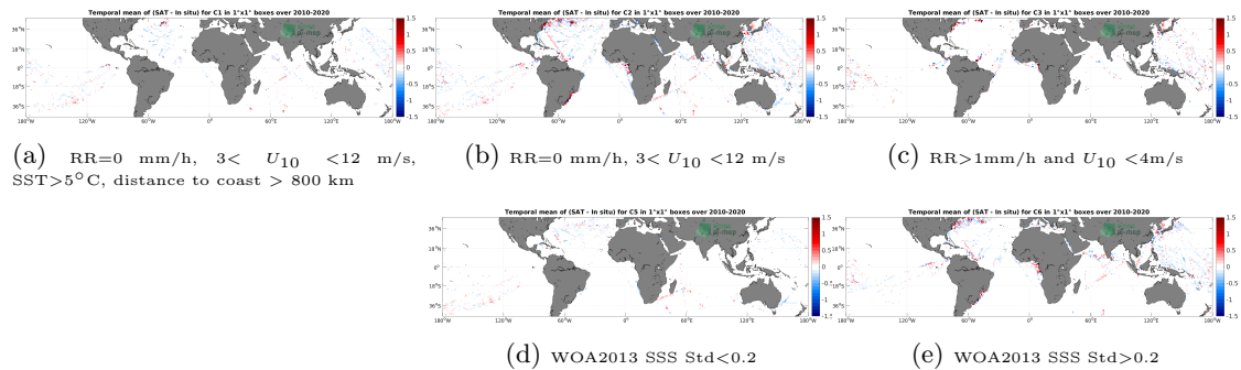
Figure 12: Temporal mean gridded over spatial boxes of size 1^\circ \times 1^\circ of \Delta SSS (CCI SSS L4 Merged-OI v3.2 - 7-day running (ESA) - TSG (LEGOS-DM)) for 5 different subdatasets corresponding to:RR=0 mm/h, 3 < U_{10} < 12 m/s, SST >5^\circ C, distance to coast > 800 km (a), RR=0 mm/h, 3 < U_{10} < 12 m/s (b), RR >1 mm/h and U_{10} < 4 m/s (c), WOA2013 SSS Std <0.2 (d), WOA2013 SSS Std >0.2 (e).
