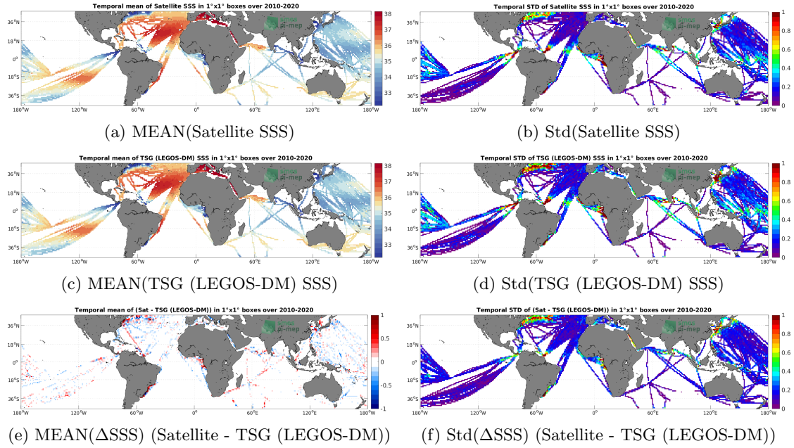
Figure 6: Temporal mean (left) and Std (right) of SSS from CCI SSS L4 Merged-OI v3.2 - 7-day running (ESA) (top), TSG (LEGOS-DM) (middle), and of \Delta SSS (Satellite - TSG (LEGOS-DM)). Only match-up pairs are used to generate these maps.
