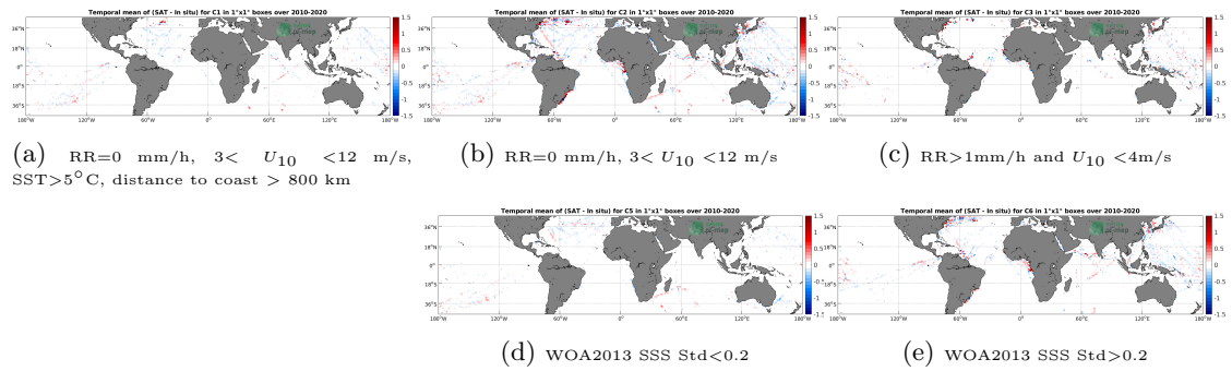
Figure 12: Temporal mean gridded over spatial boxes of size 1°x1° of \Delta SSS (CCI SSS L4 Merged-OI v3.2 - 7-day running (ESA) - TSG (LEGOS-DM)) for 5 different subdatasets corresponding to:RR=0 mm/h, 3 < U_{10} < 12 m/s, SST>5°C, distance to coast > 800 km (a), RR=0 mm/h, 3 < U_{10} < 12 m/s (b), RR>1mm/h and U_{10} < 4 m/s (c), WOA2013 SSS Std<0.2 (d), WOA2013 SSS Std>0.2 (e).
