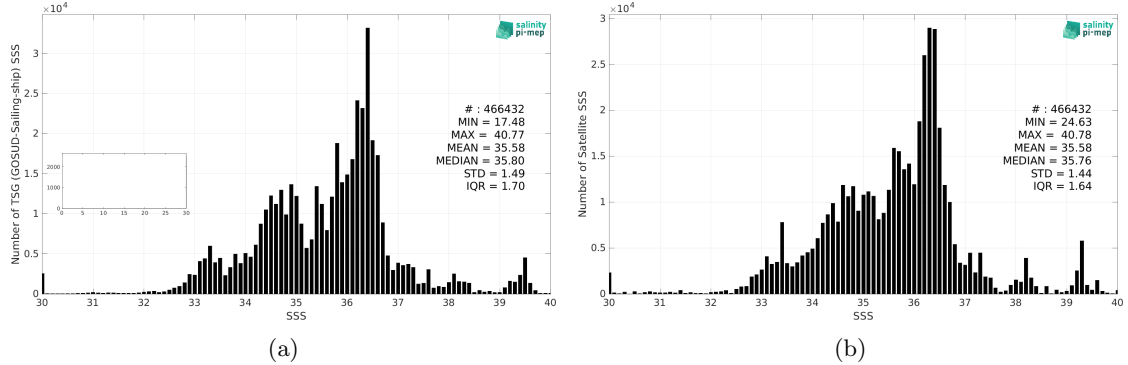
Figure 2: Histograms of SSS from TSG (GOSUD-Sailing-ship) (a) and CCI SSS L4 Merged-OI v3.2 - 7-day running (ESA) (b) considering all match-up pairs per bins of 0.1 over the Mid-Low Latitudes 45N-45S Pi-MEP region and for the full satellite product period.
