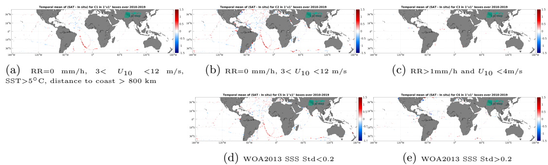
Figure 12: Temporal mean gridded over spatial boxes of size 1^\circ \times 1^\circ of \Delta SSS (CCI SSS L4 Merged-OI v3.2 - 7-day running (ESA) - TSG (GOSUD-Sailing-ship)) for 5 different subdatasets corresponding to: RR=0 mm/h, 3 < U_{10} < 12 m/s, SST > 5^\circ\text{C} , distance to coast > 800 km (a), RR=0 mm/h, 3 < U_{10} < 12 m/s (b), RR > 1 mm/h and U_{10} < 4 m/s (c), WOA2013 SSS Std < 0.2 (d), WOA2013 SSS Std > 0.2 (e).
