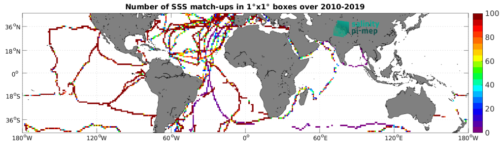
Figure 4: Number of SSS match-ups between TSG (GOSUD-Sailing-ship) SSS and the CCI SSS L4 Merged-OI v3.2 - 7-day running (ESA) SSS product for the Mid-Low Latitudes 45N-45S Pi-MEP region over 1^\circ \times 1^\circ boxes and for the full satellite product period.
