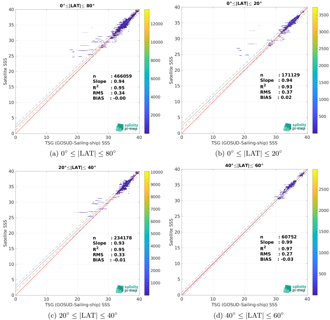
Figure 9: Contour maps of the concentration of CCI SSS L4 Merged-OI v3.2 - 7-day running (ESA) SSS (y-axis) versus TSG (GOSUD-Sailing-ship) SSS (x-axis) at match-up pairs for different latitude bands. For each plot, the red line shows x=y . The black thin and dashed lines indicate a linear fit through the data cloud and the \pm 95\% confidence levels, respectively. The number match-up pairs n , the slope and R^2 coefficient of the linear fit, the root mean square (RMS) and the mean bias between satellite and in situ data are indicated for each latitude band in each plots.
