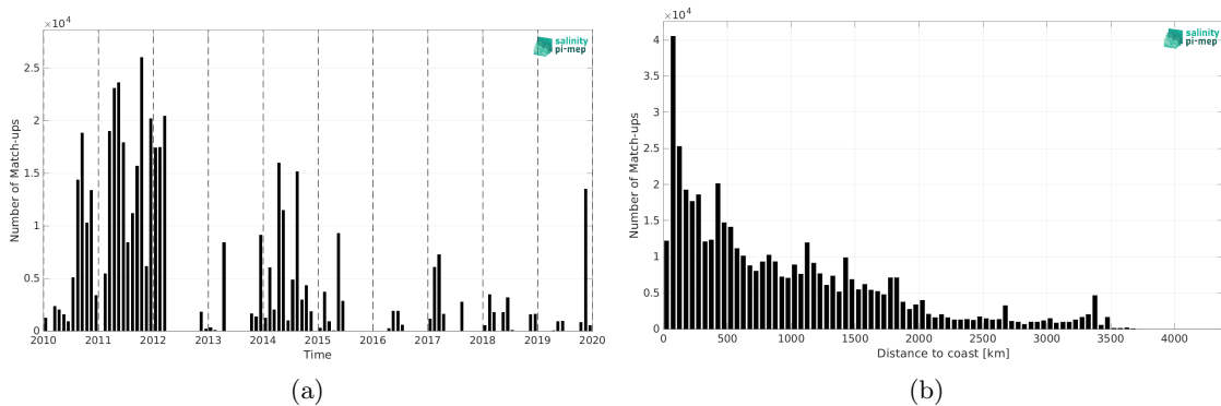
Figure 1: Number of match-ups between TSG (GOSUD-Sailing-ship) and CCI SSS L4 Merged-OI v3.2 - 7-day running (ESA) SSS as a function of time (a) and as function of the distance to coast (b) over the Mid-Low Latitudes 45N-45S Pi-MEP region and for the full satellite product period.
