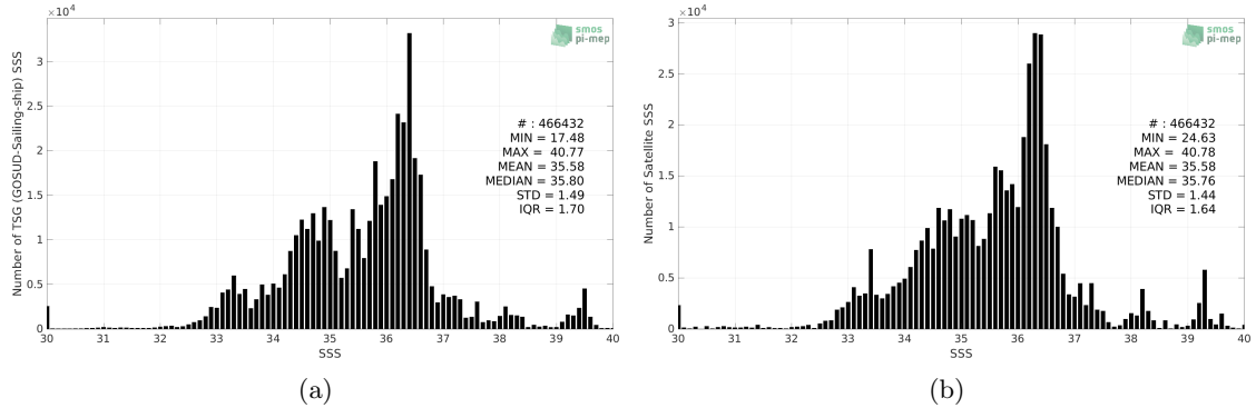
Figure 2: Histograms of SSS from TSG (GOSUD-Sailing-ship) (a) and CCI SSS L4 Merged-OI v3.2 - 7-day running (ESA) (b) considering all match-up pairs per bins of 0.1 over the Mid-Low Latitudes 45N-45S Pi-MEP region and for the full satellite product period.
