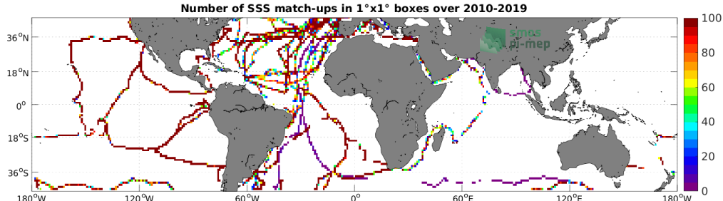
Figure 4: Number of SSS match-ups between TSG (GOSUD-Sailing-ship) SSS and the CCI SSS L4 Merged-OI v3.2 - 7-day running (ESA) SSS product for the Mid-Low Latitudes 45N-45S Pi-MEP region over 1^\circ \times 1^\circ boxes and for the full satellite product period.
