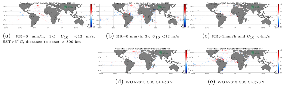
Figure 12: Temporal mean gridded over spatial boxes of size 1^\circ \times 1^\circ of \Delta\text{SSS} (CCI SSS L4 Merged-OI v3.2 - 7-day running (ESA) - TSG (GOSUD-Research-vessel)) for 5 different subdatasets corresponding to: RR=0 mm/h, 3 < U_{10} < 12 m/s, SST > 5°C, distance to coast > 800 km (a), RR=0 mm/h, 3 < U_{10} < 12 m/s (b), RR > 1mm/h and U_{10} < 4 m/s (c), WOA2013 SSS Std < 0.2 (d), WOA2013 SSS Std > 0.2 (e).
