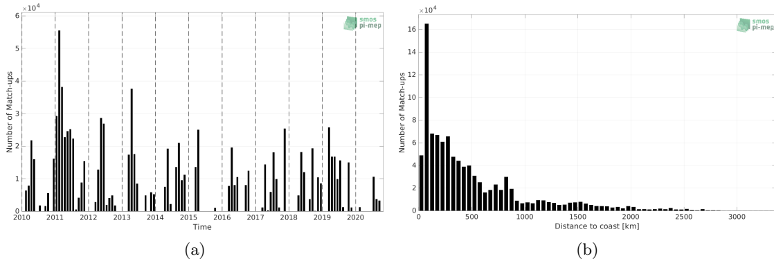
Figure 1: Number of match-ups between TSG (CSIC-UTM) and CCI SSS L4 Merged-OI v3.2 - 7-day running (ESA) SSS as a function of time (a) and as function of the distance to coast (b) over the Mid-Low Latitudes 45N-45S Pi-MEP region and for the full satellite product period.
