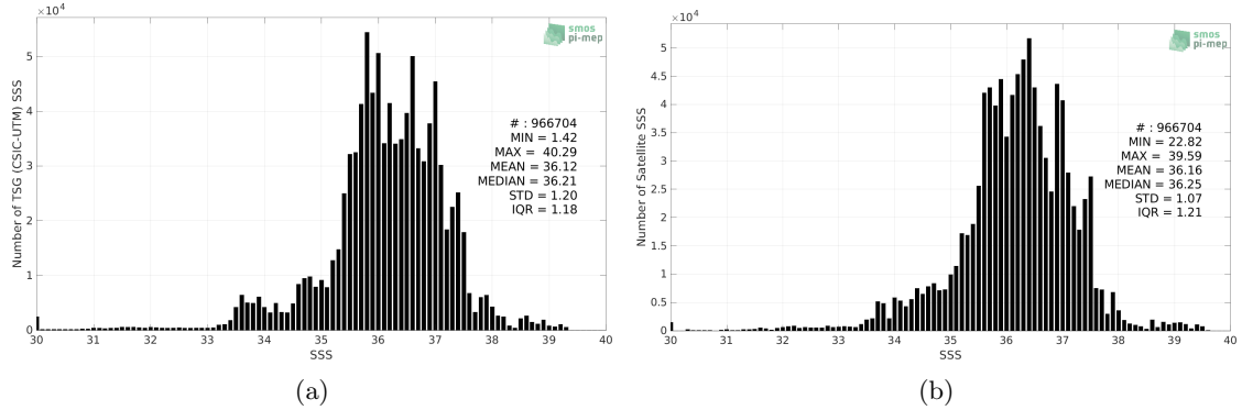
Figure 2: Histograms of SSS from TSG (CSIC-UTM) (a) and CCI SSS L4 Merged-OI v3.2 - 7-day running (ESA) (b) considering all match-up pairs per bins of 0.1 over the Mid-Low Latitudes 45N-45S Pi-MEP region and for the full satellite product period.
