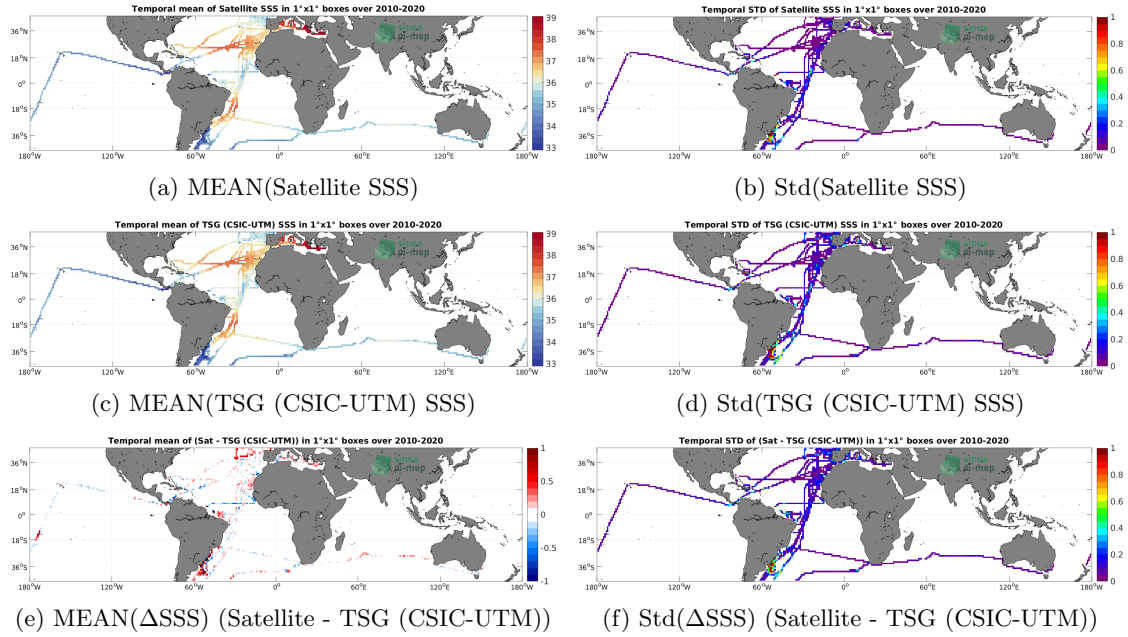
Figure 6: Temporal mean (left) and Std (right) of SSS from CCI SSS L4 Merged-OI v3.2 - 7-day running (ESA) (top), TSG (CSIC-UTM) (middle), and of \Delta SSS (Satellite - TSG (CSIC-UTM)). Only match-up pairs are used to generate these maps.
