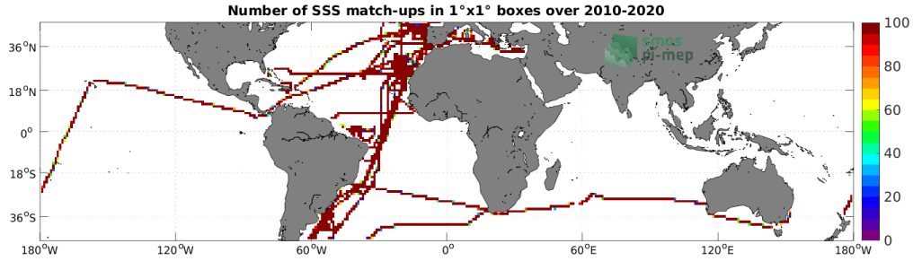
Figure 4: Number of SSS match-ups between TSG (CSIC-UTM) SSS and the CCI SSS L4 Merged-OI v3.2 - 7-day running (ESA) SSS product for the Mid-Low Latitudes 45N-45S Pi-MEP region over 1^\circ \times 1^\circ boxes and for the full satellite product period.
