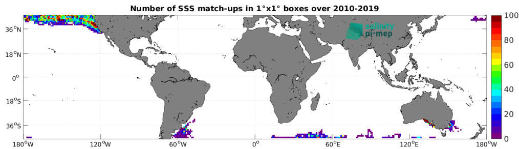
Figure 4: Number of SSS match-ups between Marine mammals SSS and the CCI SSS L4 Merged-OI v3.2 - 7-day running (ESA) SSS product for the Mid-Low Latitudes 45N-45S Pi-MEP region over 1^\circ \times 1^\circ boxes and for the full satellite product period.
