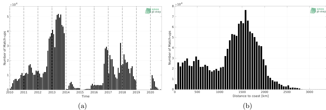
Figure 1: Number of match-ups between Surface drifters and CCI SSS L4 Merged-OI v3.2 - 7-day running (ESA) SSS as a function of time (a) and as function of the distance to coast (b) over the Mid-Low Latitudes 45N-45S Pi-MEP region and for the full satellite product period.
