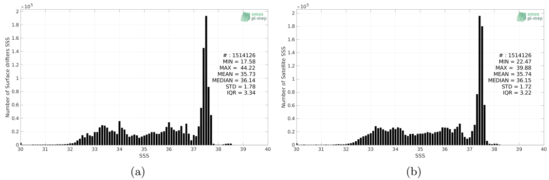
Figure 2: Histograms of SSS from Surface drifters (a) and CCI SSS L4 Merged-OI v3.2 - 7-day running (ESA) (b) considering all match-up pairs per bins of 0.1 over the Mid-Low Latitudes 45N-45S Pi-MEP region and for the full satellite product period.
