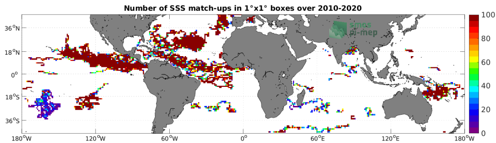
Figure 3: Number of SSS match-ups between Surface drifters SSS and the CCI SSS L4 Merged-OI v3.2 - 7-day running (ESA) SSS product for the Mid-Low Latitudes 45N-45S Pi-MEP region over 1^\circ \times 1^\circ boxes and for the full satellite product period.
