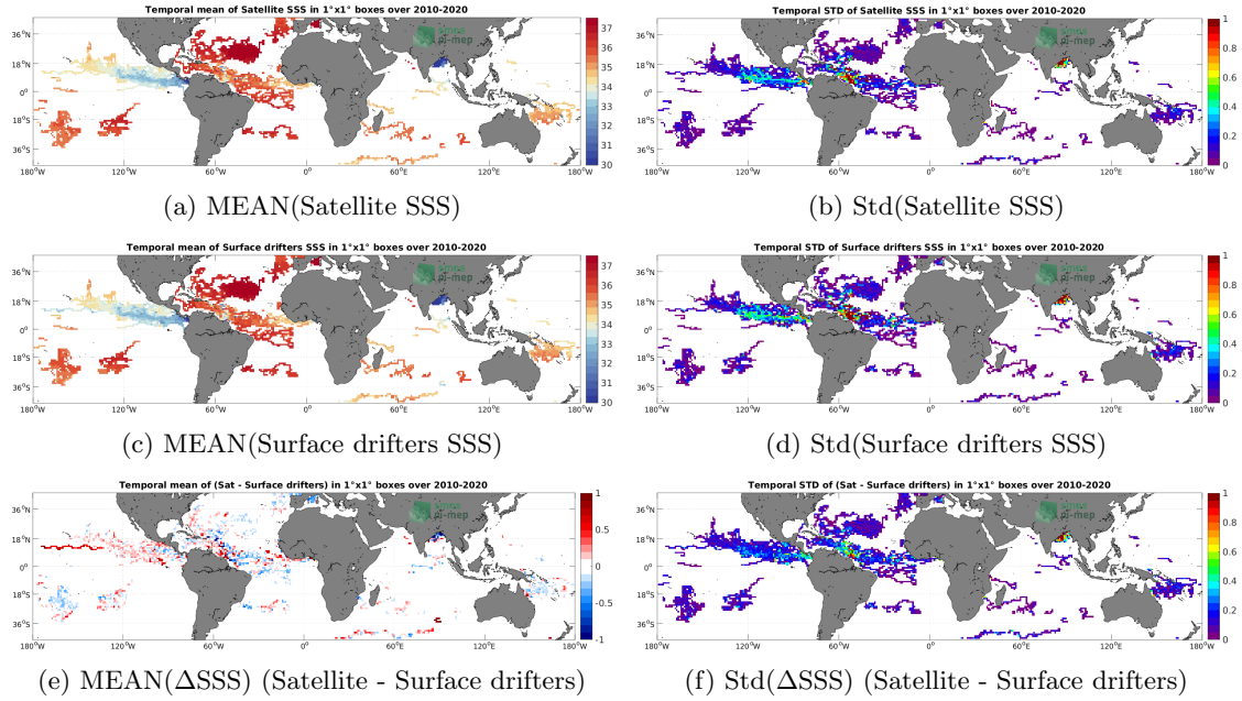
Figure 5: Temporal mean (left) and Std (right) of SSS from CCI SSS L4 Merged-OI v3.2 - 7-day running (ESA) (top), Surface drifters (middle), and of \Delta SSS (Satellite - Surface drifters). Only match-up pairs are used to generate these maps.
