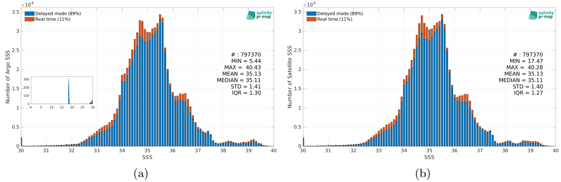
Figure 2: Histograms of SSS from Argo (a) and CCI SSS L4 Merged-OI v3.2 - 7-day running (ESA) (b) considering all match-up pairs per bins of 0.1 over the Mid-Low Latitudes 45N-45S Pi-MEP region and for the full satellite product period.
