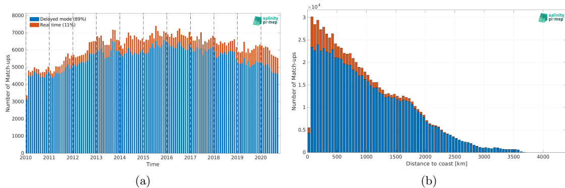
Figure 1: Number of match-ups between Argo and CCI SSS L4 Merged-OI v3.2 - 7-day running (ESA) SSS as a function of time (a) and as function of the distance to coast (b) over the Mid-Low Latitudes 45N-45S Pi-MEP region and for the full satellite product period.
