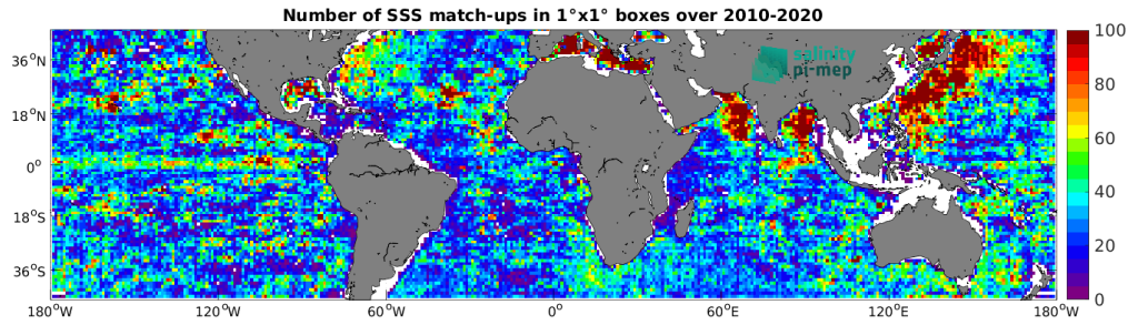
Figure 4: Number of SSS match-ups between Argo SSS and the CCI SSS L4 Merged-OI v3.2 - 7-day running (ESA) SSS product for the Mid-Low Latitudes 45N-45S Pi-MEP region over 1^\circ \times 1^\circ boxes and for the full satellite product period.
