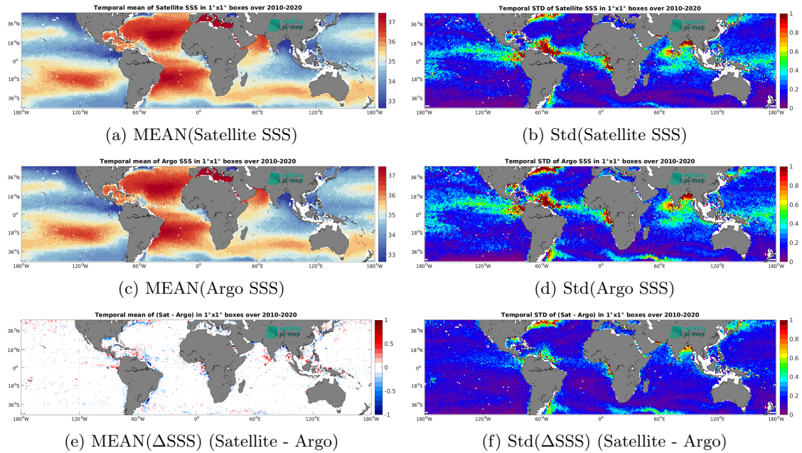
Figure 6: Temporal mean (left) and Std (right) of SSS from CCI SSS L4 Merged-OI v3.2 - 7-day running (ESA) (top), Argo (middle), and of \Delta SSS (Satellite - Argo). Only match-up pairs are used to generate these maps.
