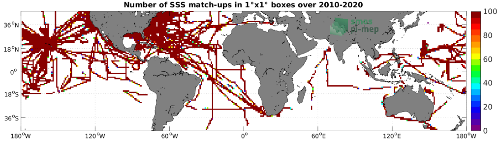
Figure 4: Number of SSS match-ups between TSG (SAMOS) SSS and the CCI SSS L4 Merged-OI v3.2 - 30-day running (ESA) SSS product for the Mid-Low Latitudes 45N-45S Pi-MEP region over 1^\circ \times 1^\circ boxes and for the full satellite product period.
