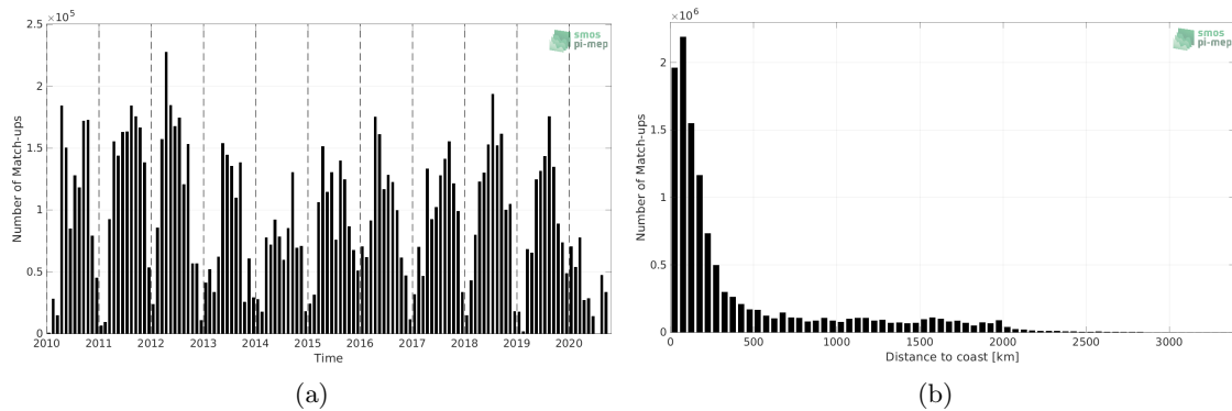
Figure 1: Number of match-ups between TSG (SAMOS) and CCI SSS L4 Merged-OI v3.2 - 30-day running (ESA) SSS as a function of time (a) and as function of the distance to coast (b) over the Mid-Low Latitudes 45N-45S Pi-MEP region and for the full satellite product period.
