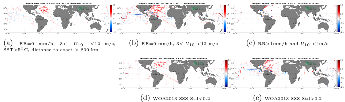
Figure 12: Temporal mean gridded over spatial boxes of size 1^\circ \times 1^\circ of \Delta SSS (CCI SSS L4 Merged-OI v3.2 - 30-day running (ESA) - TSG (SAMOS)) for 5 different subdatasets corresponding to:RR=0 mm/h, 3 < U_{10} < 12 m/s, SST >5^\circ C, distance to coast > 800 km (a), RR=0 mm/h, 3 < U_{10} < 12 m/s (b), RR >1 mm/h and U_{10} < 4 m/s (c), WOA2013 SSS Std <0.2 (d), WOA2013 SSS Std >0.2 (e).
