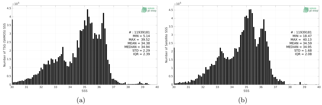
Figure 2: Histograms of SSS from TSG (SAMOS) (a) and CCI SSS L4 Merged-OI v3.2 - 30-day running (ESA) (b) considering all match-up pairs per bins of 0.1 over the Mid-Low Latitudes 45N-45S Pi-MEP region and for the full satellite product period.
