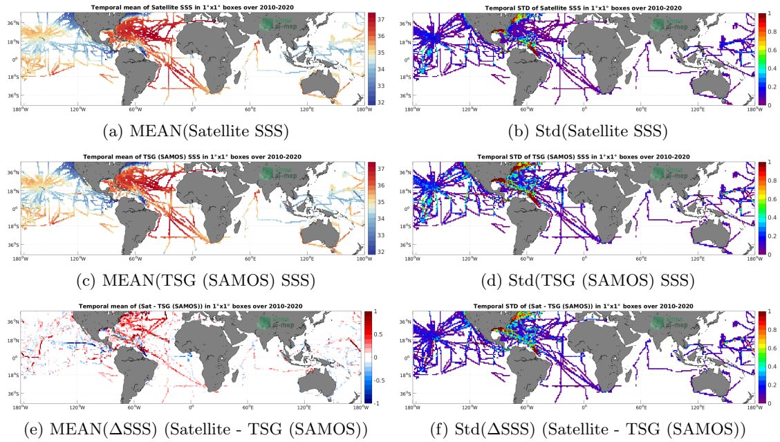
Figure 6: Temporal mean (left) and Std (right) of SSS from CCI SSS L4 Merged-OI v3.2 - 30-day running (ESA) (top), TSG (SAMOS) (middle), and of \Delta SSS (Satellite - TSG (SAMOS)). Only match-up pairs are used to generate these maps.
