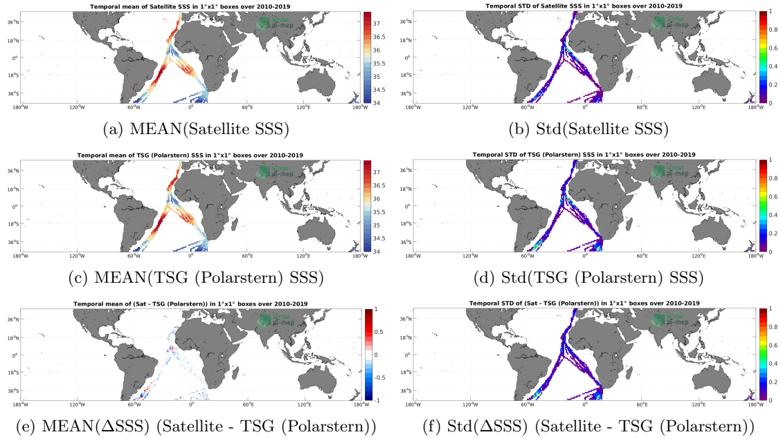
Figure 6: Temporal mean (left) and Std (right) of SSS from CCI SSS L4 Merged-OI v3.2 - 30-day running (ESA) (top), TSG (Polarstern) (middle), and of \Delta SSS (Satellite - TSG (Polarstern)). Only match-up pairs are used to generate these maps.
