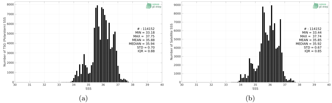
Figure 2: Histograms of SSS from TSG (Polarstern) (a) and CCI SSS L4 Merged-OI v3.2 - 30-day running (ESA) (b) considering all match-up pairs per bins of 0.1 over the Mid-Low Latitudes 45N-45S Pi-MEP region and for the full satellite product period.
