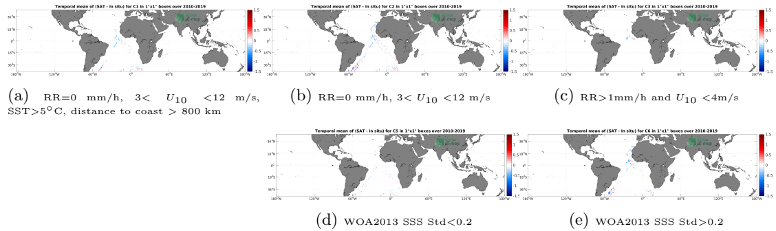
Figure 12: Temporal mean gridded over spatial boxes of size 1^\circ \times 1^\circ of \Delta\text{SSS} (CCI SSS L4 Merged-OI v3.2 - 30-day running (ESA) - TSG (Polarstern)) for 5 different subdatasets corresponding to:RR=0 mm/h, 3 < U_{10} < 12 m/s, SST >5^\circ\text{C} , distance to coast > 800 km (a), RR=0 mm/h, 3 < U_{10} < 12 m/s (b), RR >1 mm/h and U_{10} < 4 m/s (c), WOA2013 SSS Std <0.2 (d), WOA2013 SSS Std >0.2 (e).
