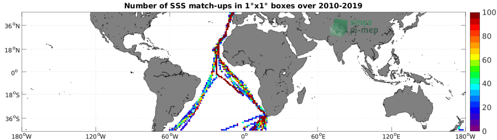
Figure 4: Number of SSS match-ups between TSG (Polarstern) SSS and the CCI SSS L4 Merged-OI v3.2 - 30-day running (ESA) SSS product for the Mid-Low Latitudes 45N-45S Pi-MEP region over 1^\circ \times 1^\circ boxes and for the full satellite product period.
