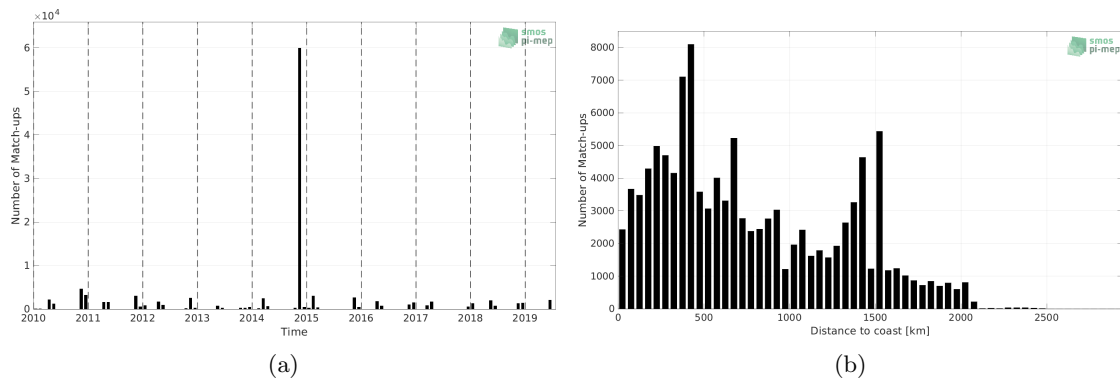
Figure 1: Number of match-ups between TSG (Polarstern) and CCI SSS L4 Merged-OI v3.2 - 30-day running (ESA) SSS as a function of time (a) and as function of the distance to coast (b) over the Mid-Low Latitudes 45N-45S Pi-MEP region and for the full satellite product period.
