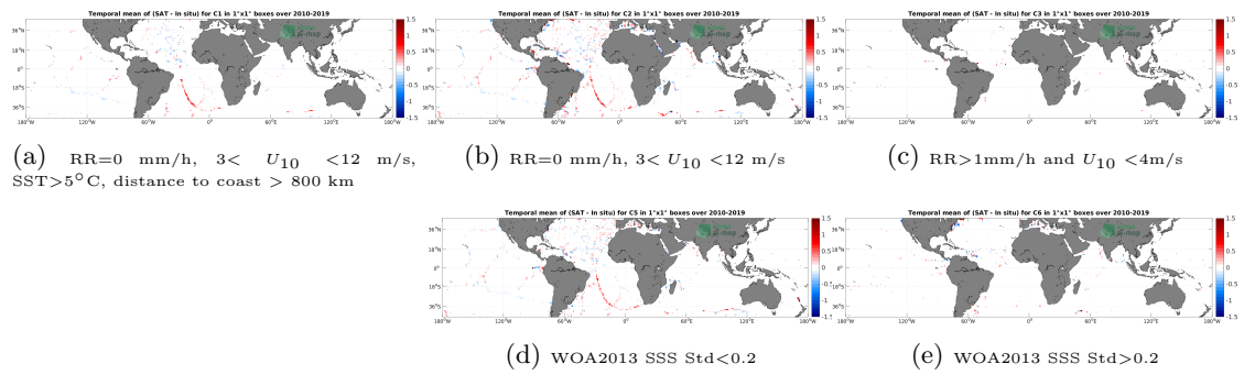
Figure 12: Temporal mean gridded over spatial boxes of size 1^\circ \times 1^\circ of \Delta SSS (CCI SSS L4 Merged-OI v3.2 - 30-day running (ESA) - TSG (GOSUD-Sailing-ship)) for 5 different subdatasets corresponding to: RR=0 mm/h, 3 < U_{10} < 12 m/s, SST > 5°C, distance to coast > 800 km (a), RR=0 mm/h, 3 < U_{10} < 12 m/s (b), RR > 1mm/h and U_{10} < 4 m/s (c), WOA2013 SSS Std < 0.2 (d), WOA2013 SSS Std > 0.2 (e).
