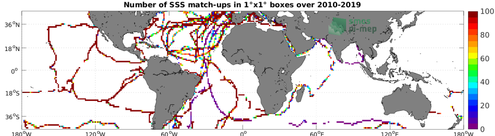
Figure 4: Number of SSS match-ups between TSG (GOSUD-Sailing-ship) SSS and the CCI SSS L4 Merged-OI v3.2 - 30-day running (ESA) SSS product for the Mid-Low Latitudes 45N-45S Pi-MEP region over 1^\circ \times 1^\circ boxes and for the full satellite product period.
