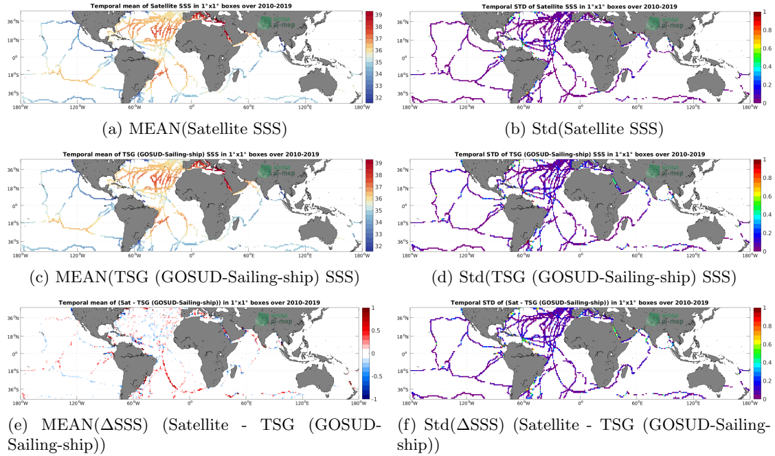
Figure 6: Temporal mean (left) and Std (right) of SSS from CCI SSS L4 Merged-OI v3.2 - 30-day running (ESA) (top), TSG (GOSUD-Sailing-ship) (middle), and of \Delta SSS (Satellite - TSG (GOSUD-Sailing-ship)). Only match-up pairs are used to generate these maps.
