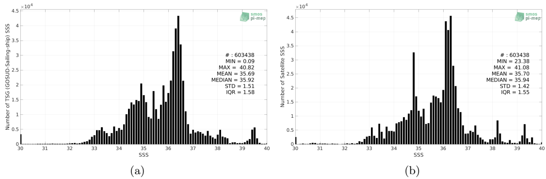
Figure 2: Histograms of SSS from TSG (GOSUD-Sailing-ship) (a) and CCI SSS L4 Merged-OI v3.2 - 30-day running (ESA) (b) considering all match-up pairs per bins of 0.1 over the Mid-Low Latitudes 45N-45S Pi-MEP region and for the full satellite product period.
