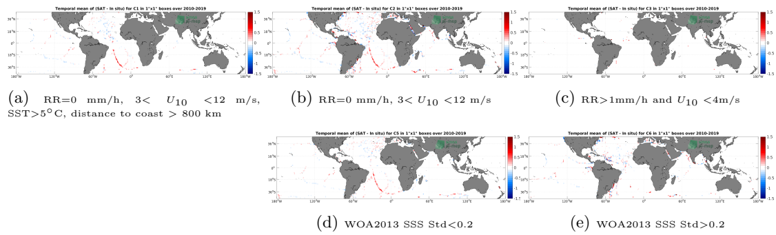
Figure 12: Temporal mean gridded over spatial boxes of size 1^\circ \times 1^\circ of \Delta\text{SSS} (CCI SSS L4 Merged-OI v3.2 - 30-day running (ESA) - TSG (GOSUD-Sailing-ship)) for 5 different subdatasets corresponding to: RR=0 mm/h, 3 < U_{10} < 12 m/s, SST > 5°C, distance to coast > 800 km (a), RR=0 mm/h, 3 < U_{10} < 12 m/s (b), RR > 1mm/h and U_{10} < 4 m/s (c), WOA2013 SSS Std < 0.2 (d), WOA2013 SSS Std > 0.2 (e).
