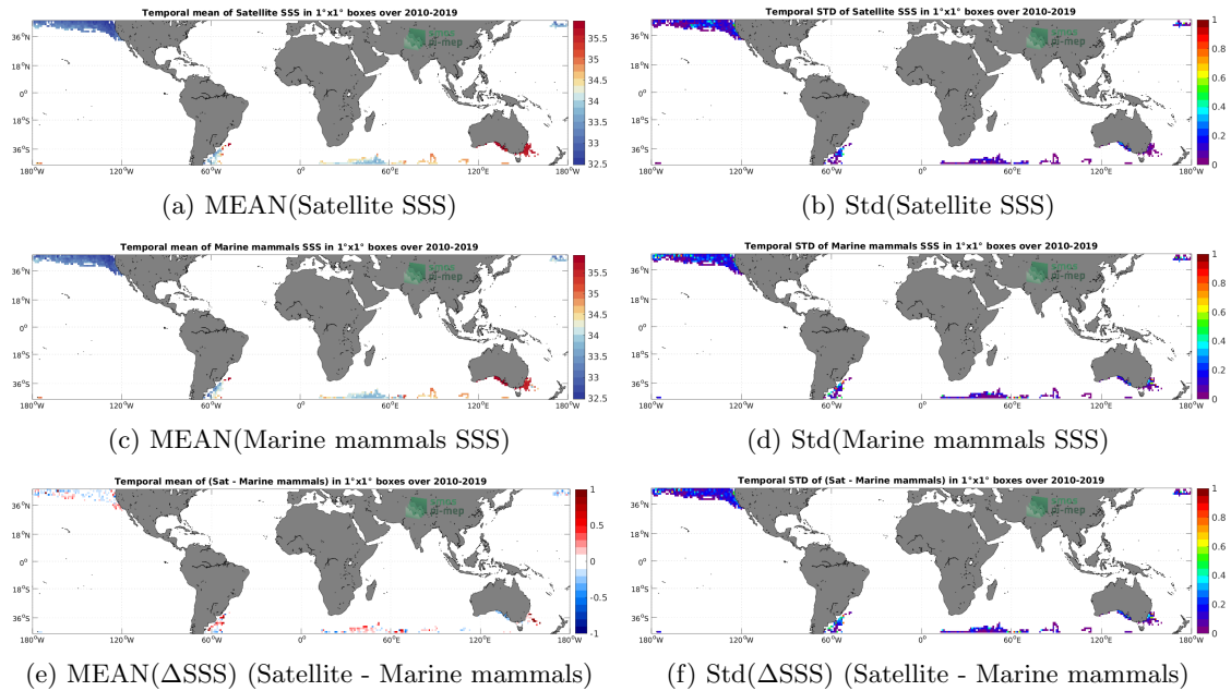
Figure 6: Temporal mean (left) and Std (right) of SSS from CCI SSS L4 Merged-OI v3.2 - 30-day running (ESA) (top), Marine mammals (middle), and of \Delta SSS (Satellite - Marine mammals). Only match-up pairs are used to generate these maps.
